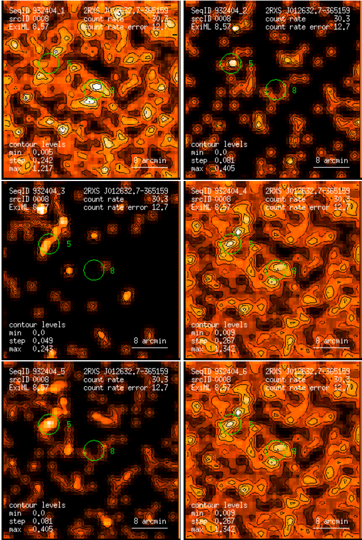
Figure 8: RASS 932404: detection 0008: band rate images, Gaussian filter: (1) PSPC channels 11 – 41, (2) 52 – 90, (3) 91 – 201, (4) 11 – 235, (5) 52 – 201, (6) 11 – 201. Broad band rates in counts/ks. Band rate contour levels in counts/ks/arcmin 2 .
