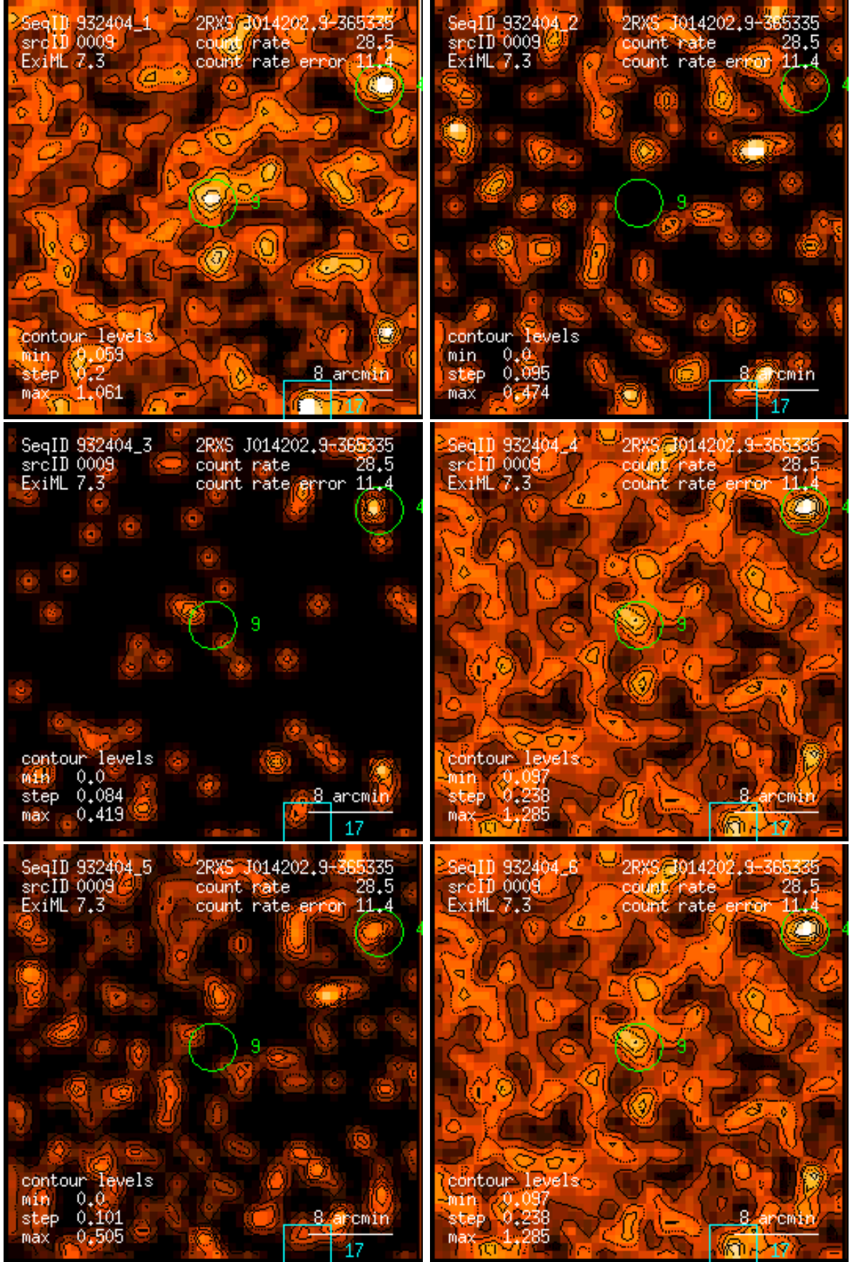
Figure 9: RASS 932404: detection 0009: band rate images, Gaussian filter: (1) PSPC channels 11 – 41, (2) 52 – 90, (3) 91 – 201, (4) 11 – 235, (5) 52 – 201, (6) 11 – 201. Broad band rates in counts/ks. Band rate contour levels in counts/ks/arcmin 2 .
