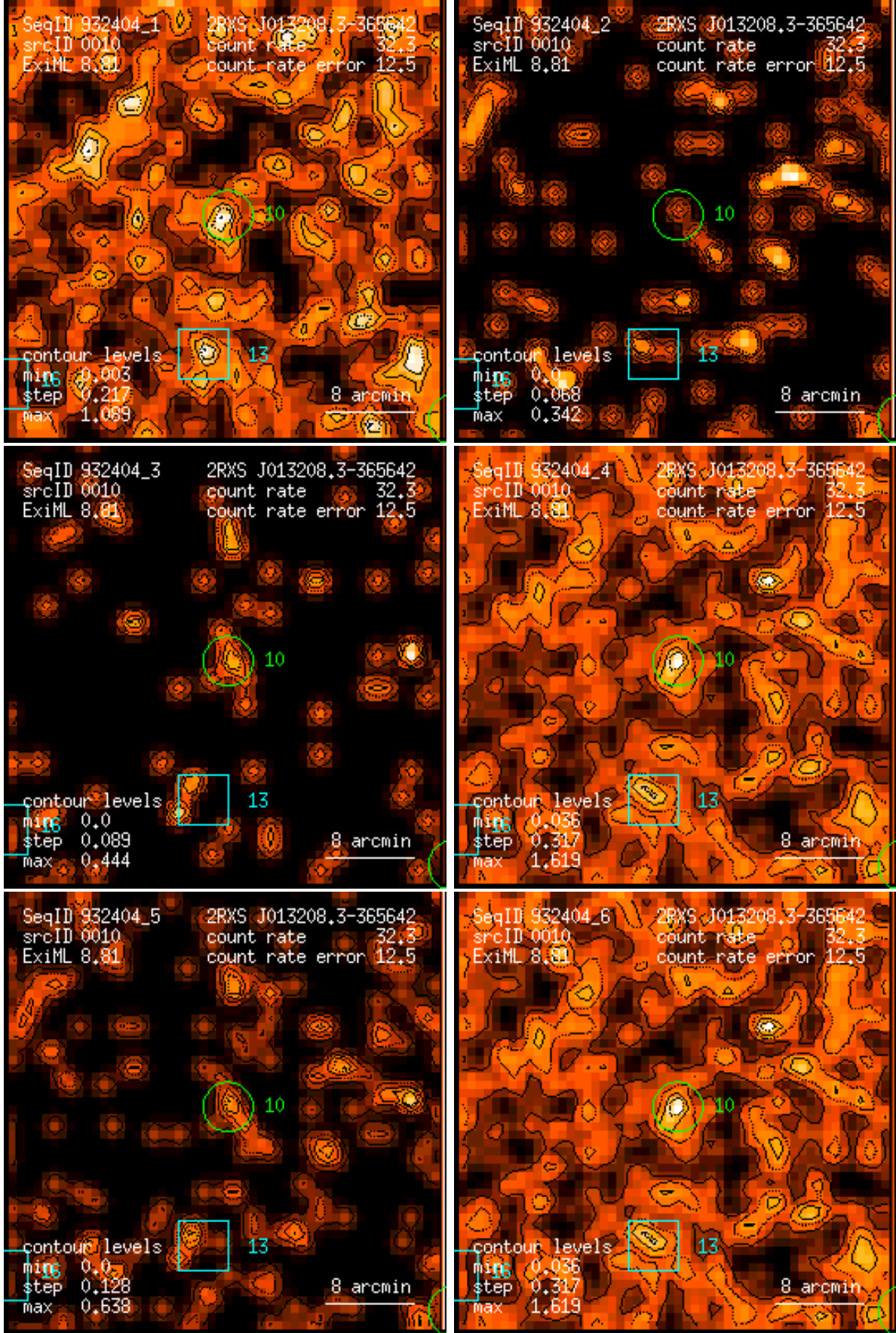
Figure 10: RASS 932404: detection 0010: band rate images, Gaussian filter: (1) PSPC channels 11 – 41, (2) 52 – 90, (3) 91 – 201, (4) 11 – 235, (5) 52 – 201, (6) 11 – 201. Broad band rates in counts/ks. Band rate contour levels in counts/ks/arcmin 2 .
