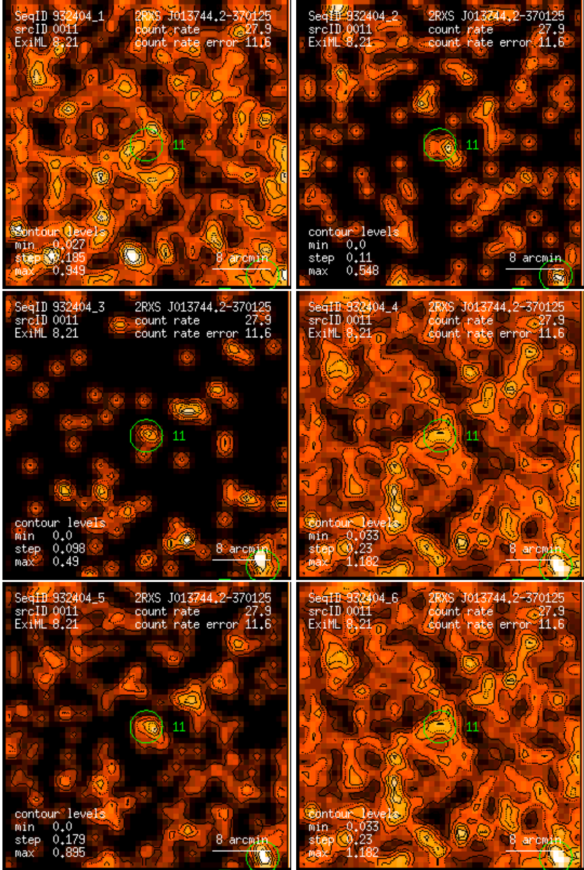
Figure 11: RASS 932404: detection 0011: band rate images, Gaussian filter: (1) PSPC channels 11 – 41, (2) 52 – 90, (3) 91 – 201, (4) 11 – 235, (5) 52 – 201, (6) 11 – 201. Broad band rates in counts/ks. Band rate contour levels in counts/ks/arcmin 2 .
