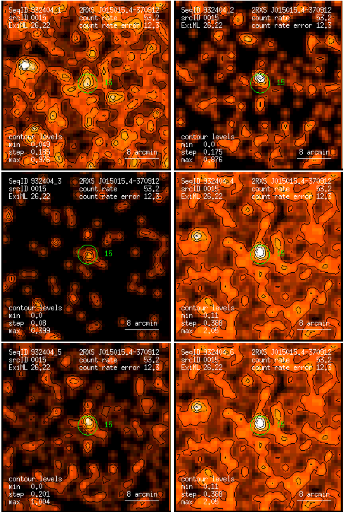
Figure 15: RASS 932404: detection 0015: band rate images, Gaussian filter: (1) PSPC channels 11 – 41, (2) 52 – 90, (3) 91 – 201, (4) 11 – 235, (5) 52 – 201, (6) 11 – 201. Broad band rates in counts/ks. Band rate contour levels in counts/ks/arcmin 2 .
