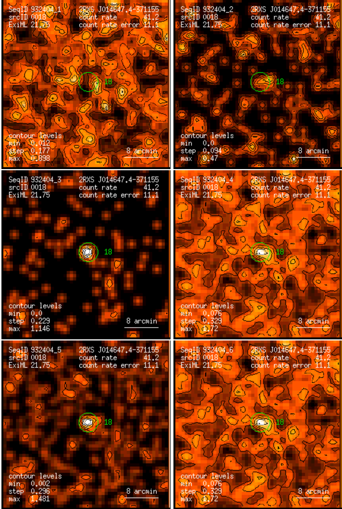
Figure 18: RASS 932404: detection 0018: band rate images, Gaussian filter: (1) PSPC channels 11 – 41, (2) 52 – 90, (3) 91 – 201, (4) 11 – 235, (5) 52 – 201, (6) 11 – 201. Broad band rates in counts/ks. Band rate contour levels in counts/ks/arcmin 2 .
