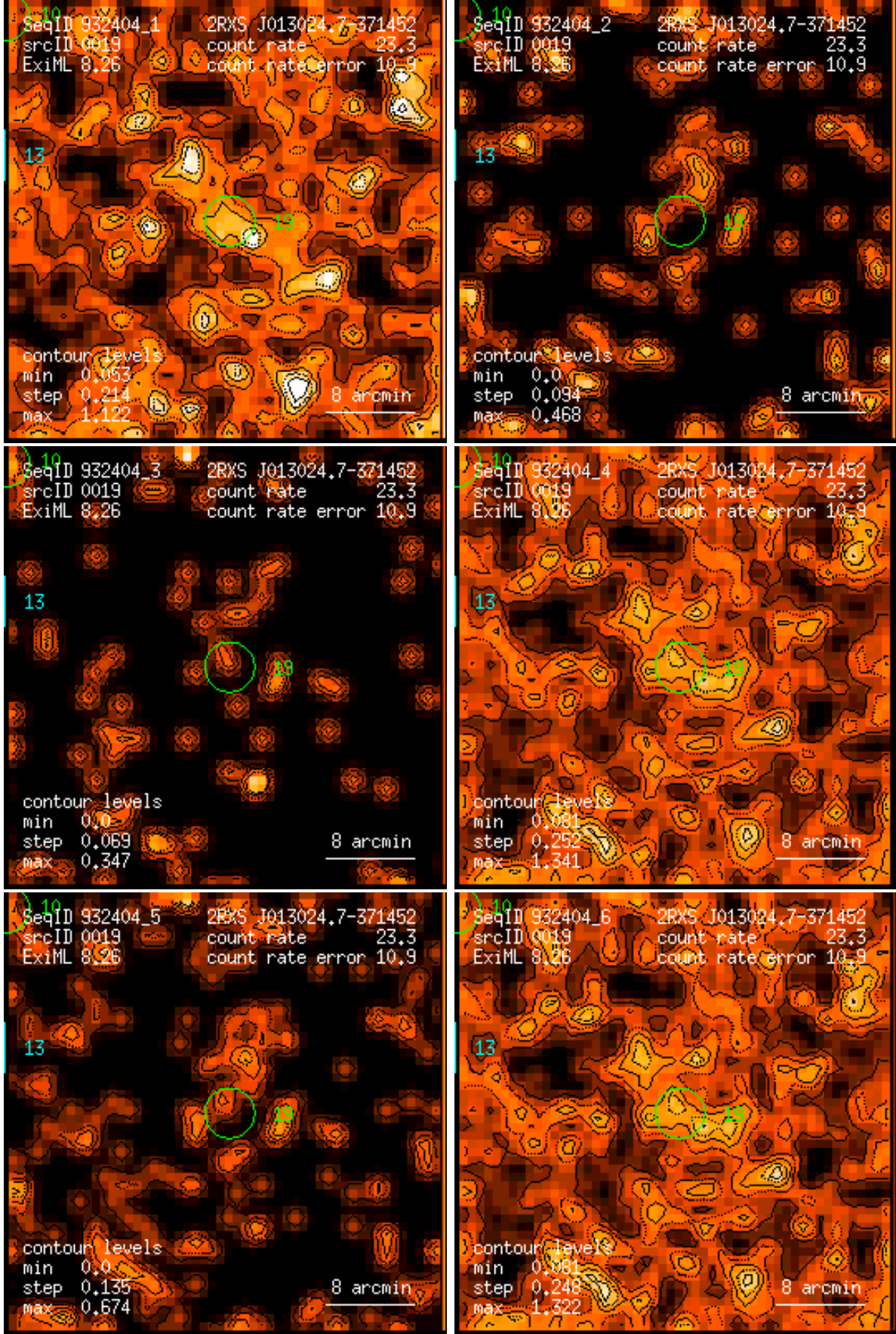
Figure 19: RASS 932404: detection 0019: band rate images, Gaussian filter: (1) PSPC channels 11 – 41, (2) 52 – 90, (3) 91 – 201, (4) 11 – 235, (5) 52 – 201, (6) 11 – 201. Broad band rates in counts/ks. Band rate contour levels in counts/ks/arcmin 2 .
