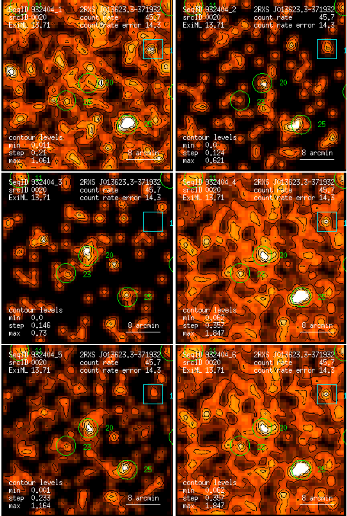
Figure 20: RASS 932404: detection 0020: band rate images, Gaussian filter: (1) PSPC channels 11 – 41, (2) 52 – 90, (3) 91 – 201, (4) 11 – 235, (5) 52 – 201, (6) 11 – 201. Broad band rates in counts/ks. Band rate contour levels in counts/ks/arcmin 2 .
