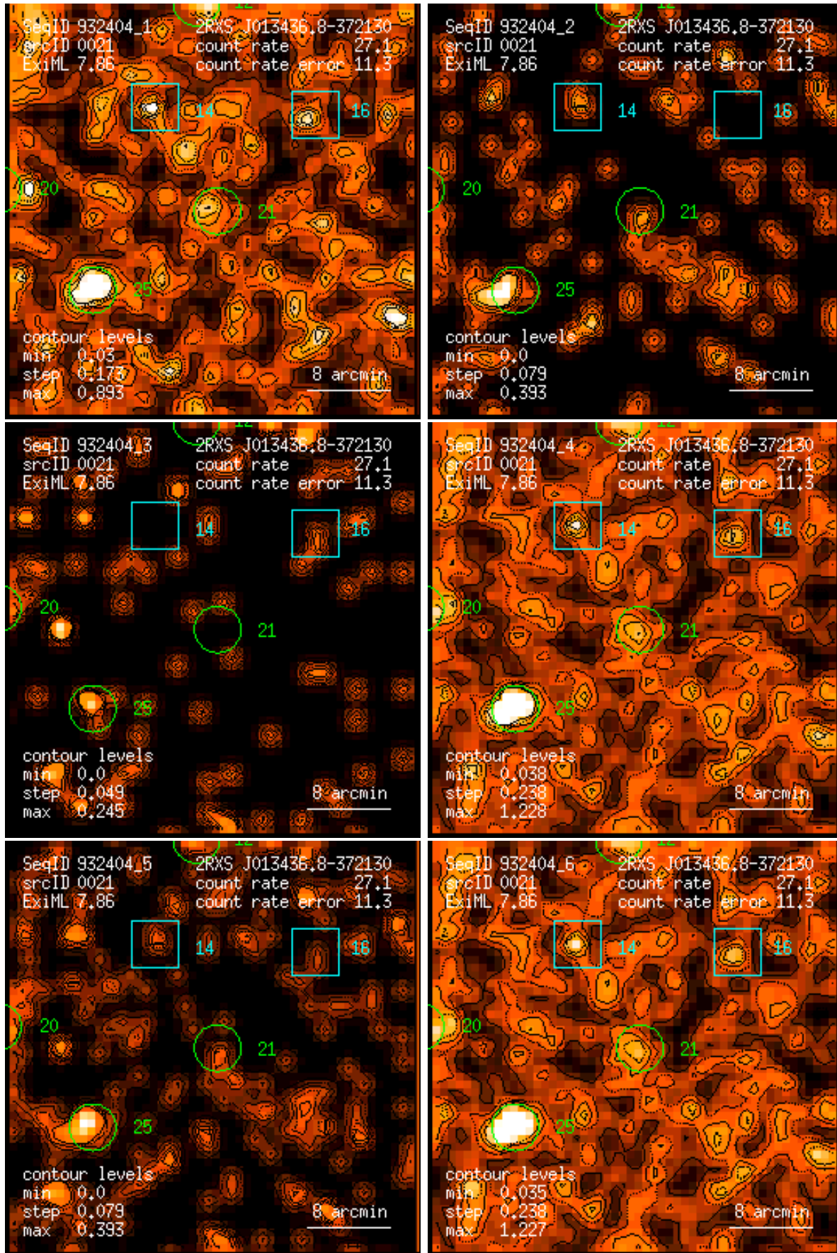
Figure 21: RASS 932404: detection 0021: band rate images, Gaussian filter: (1) PSPC channels 11 – 41, (2) 52 – 90, (3) 91 – 201, (4) 11 – 235, (5) 52 – 201, (6) 11 – 201. Broad band rates in counts/ks. Band rate contour levels in counts/ks/arcmin 2 .
