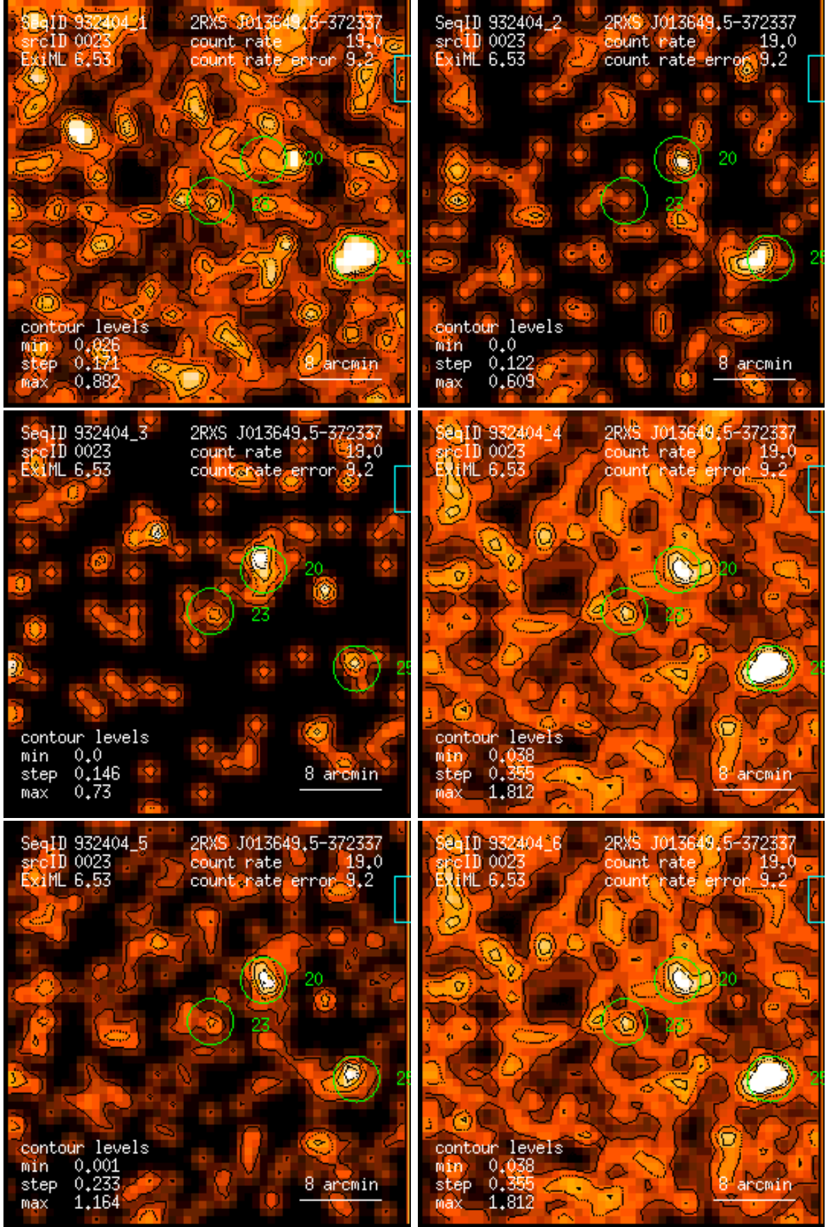
Figure 23: RASS 932404: detection 0023: band rate images, Gaussian filter: (1) PSPC channels 11 – 41, (2) 52 – 90, (3) 91 – 201, (4) 11 – 235, (5) 52 – 201, (6) 11 – 201. Broad band rates in counts/ks. Band rate contour levels in counts/ks/arcmin 2 .
