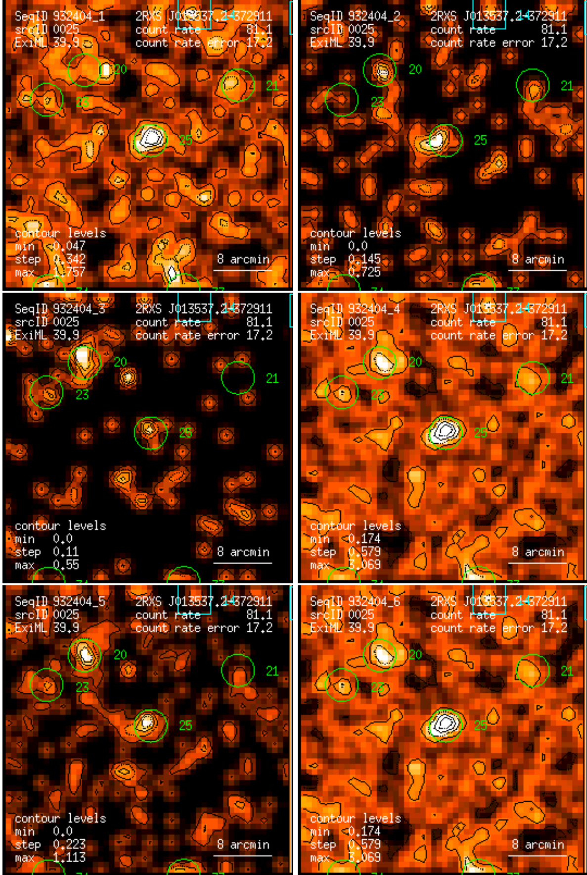
Figure 25: RASS 932404: detection 0025: band rate images, Gaussian filter: (1) PSPC channels 11 – 41, (2) 52 – 90, (3) 91 – 201, (4) 11 – 235, (5) 52 – 201, (6) 11 – 201. Broad band rates in counts/ks. Band rate contour levels in counts/ks/arcmin 2 .
