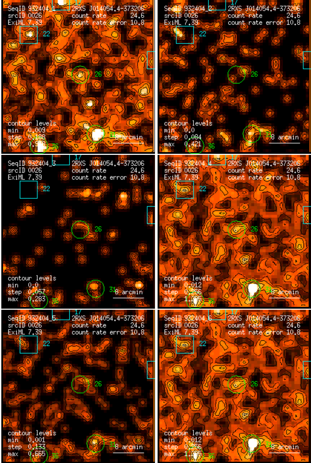
Figure 26: RASS 932404: detection 0026: band rate images, Gaussian filter: (1) PSPC channels 11 – 41, (2) 52 – 90, (3) 91 – 201, (4) 11 – 235, (5) 52 – 201, (6) 11 – 201. Broad band rates in counts/ks. Band rate contour levels in counts/ks/arcmin 2 .
