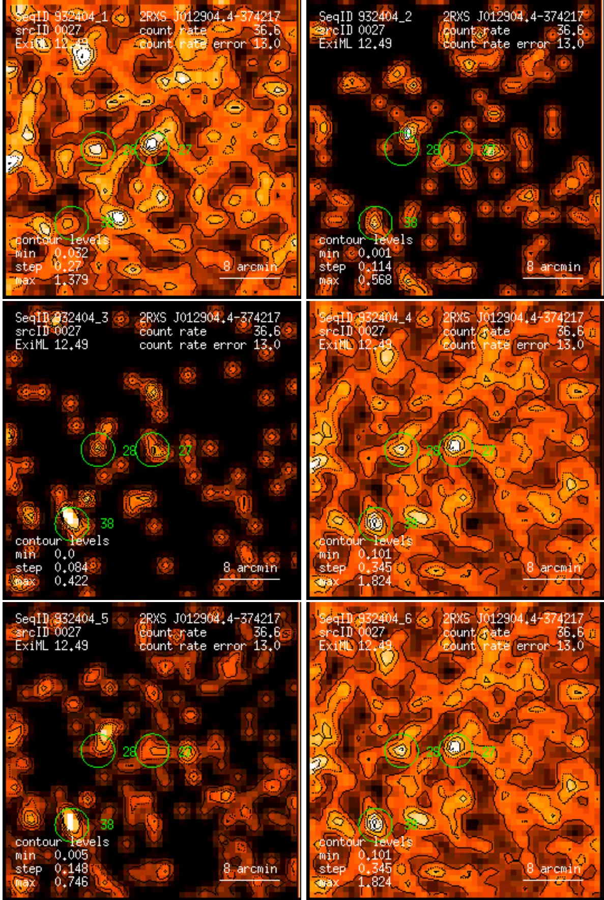
Figure 27: RASS 932404: detection 0027: band rate images, Gaussian filter: (1) PSPC channels 11 – 41, (2) 52 – 90, (3) 91 – 201, (4) 11 – 235, (5) 52 – 201, (6) 11 – 201. Broad band rates in counts/ks. Band rate contour levels in counts/ks/arcmin 2 .
