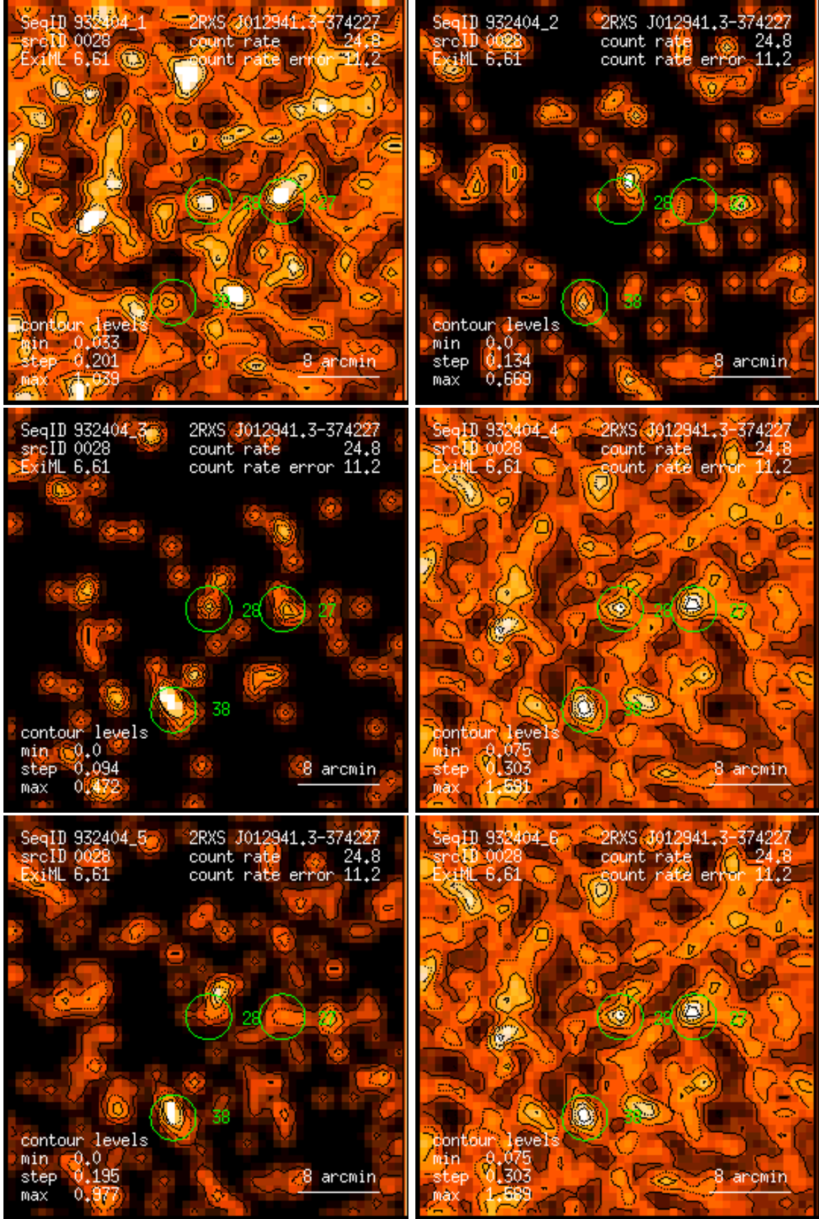
Figure 28: RASS 932404: detection 0028: band rate images, Gaussian filter: (1) PSPC channels 11 – 41, (2) 52 – 90, (3) 91 – 201, (4) 11 – 235, (5) 52 – 201, (6) 11 – 201. Broad band rates in counts/ks. Band rate contour levels in counts/ks/arcmin 2 .
