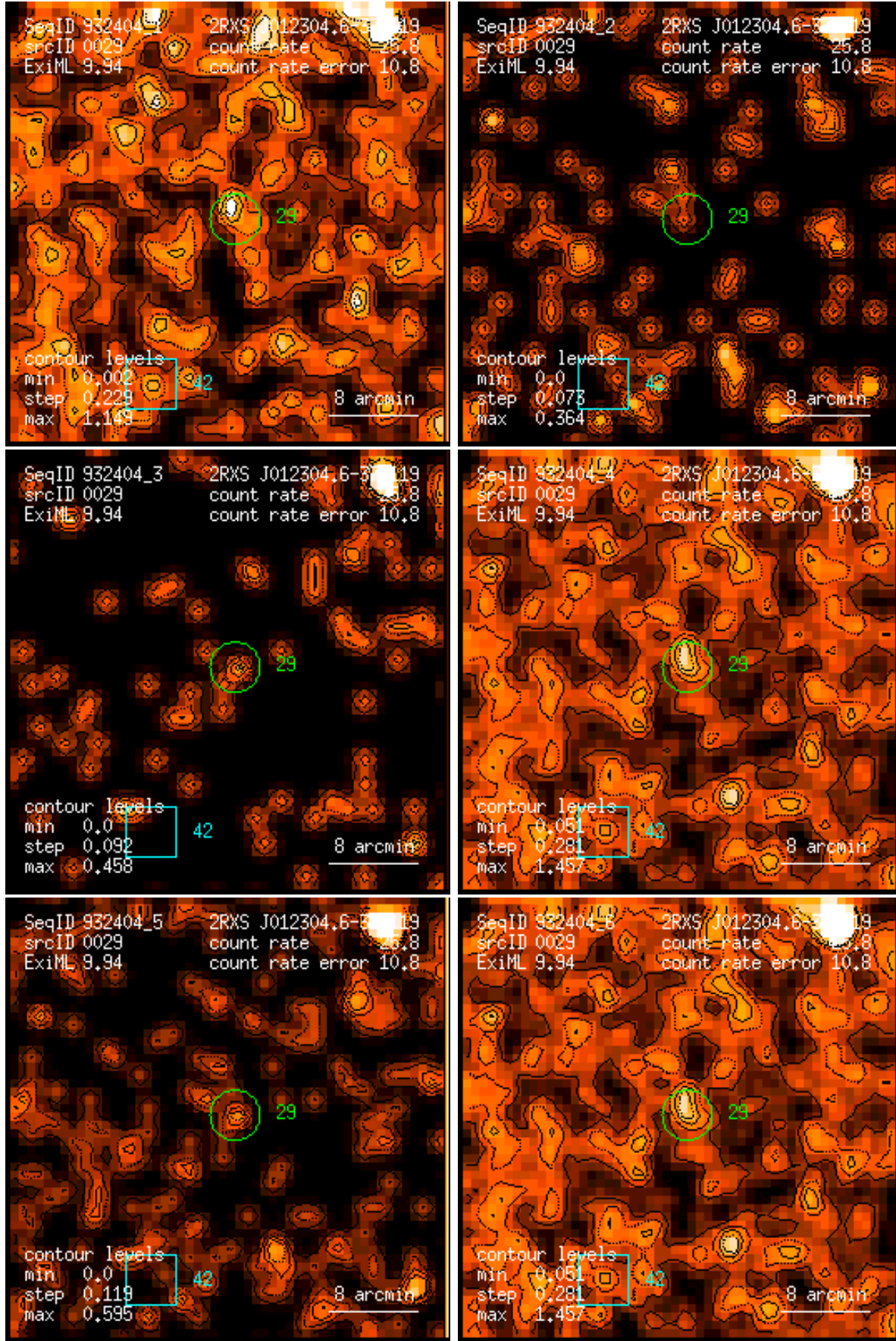
Figure 29: RASS 932404: detection 0029: band rate images, Gaussian filter: (1) PSPC channels 11 – 41, (2) 52 – 90, (3) 91 – 201, (4) 11 – 235, (5) 52 – 201, (6) 11 – 201. Broad band rates in counts/ks. Band rate contour levels in counts/ks/arcmin 2 .
