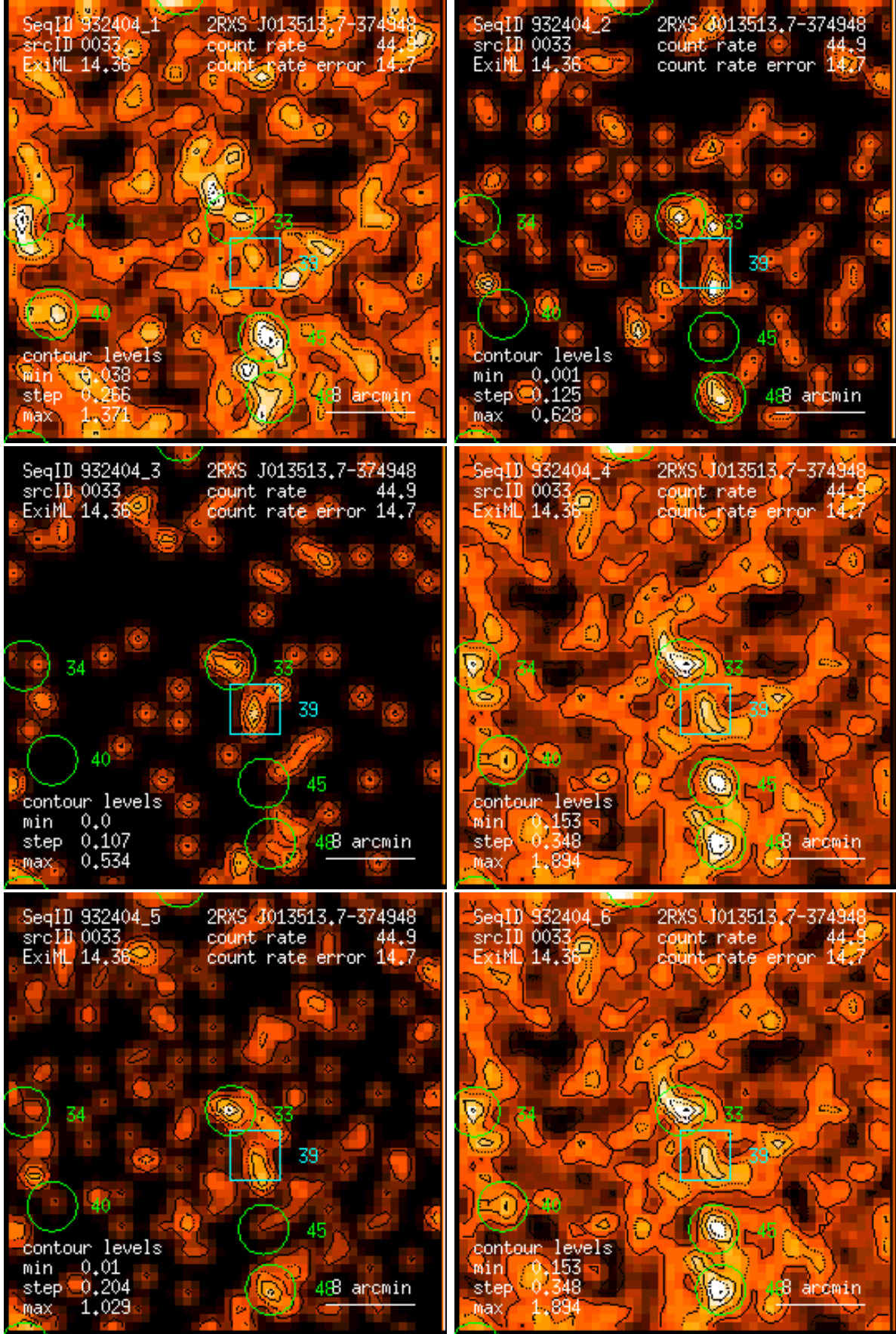
Figure 33: RASS 932404: detection 0033: band rate images, Gaussian filter: (1) PSPC channels 11 – 41, (2) 52 – 90, (3) 91 – 201, (4) 11 – 235, (5) 52 – 201, (6) 11 – 201. Broad band rates in counts/ks. Band rate contour levels in counts/ks/arcmin 2 .
