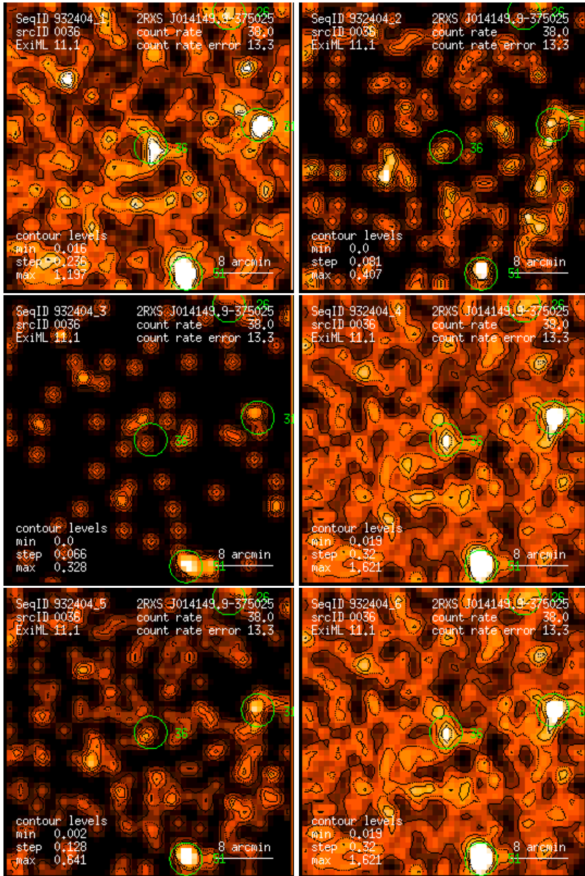
Figure 36: RASS 932404: detection 0036: band rate images, Gaussian filter: (1) PSPC channels 11 – 41, (2) 52 – 90, (3) 91 – 201, (4) 11 – 235, (5) 52 – 201, (6) 11 – 201. Broad band rates in counts/ks. Band rate contour levels in counts/ks/arcmin 2 .
