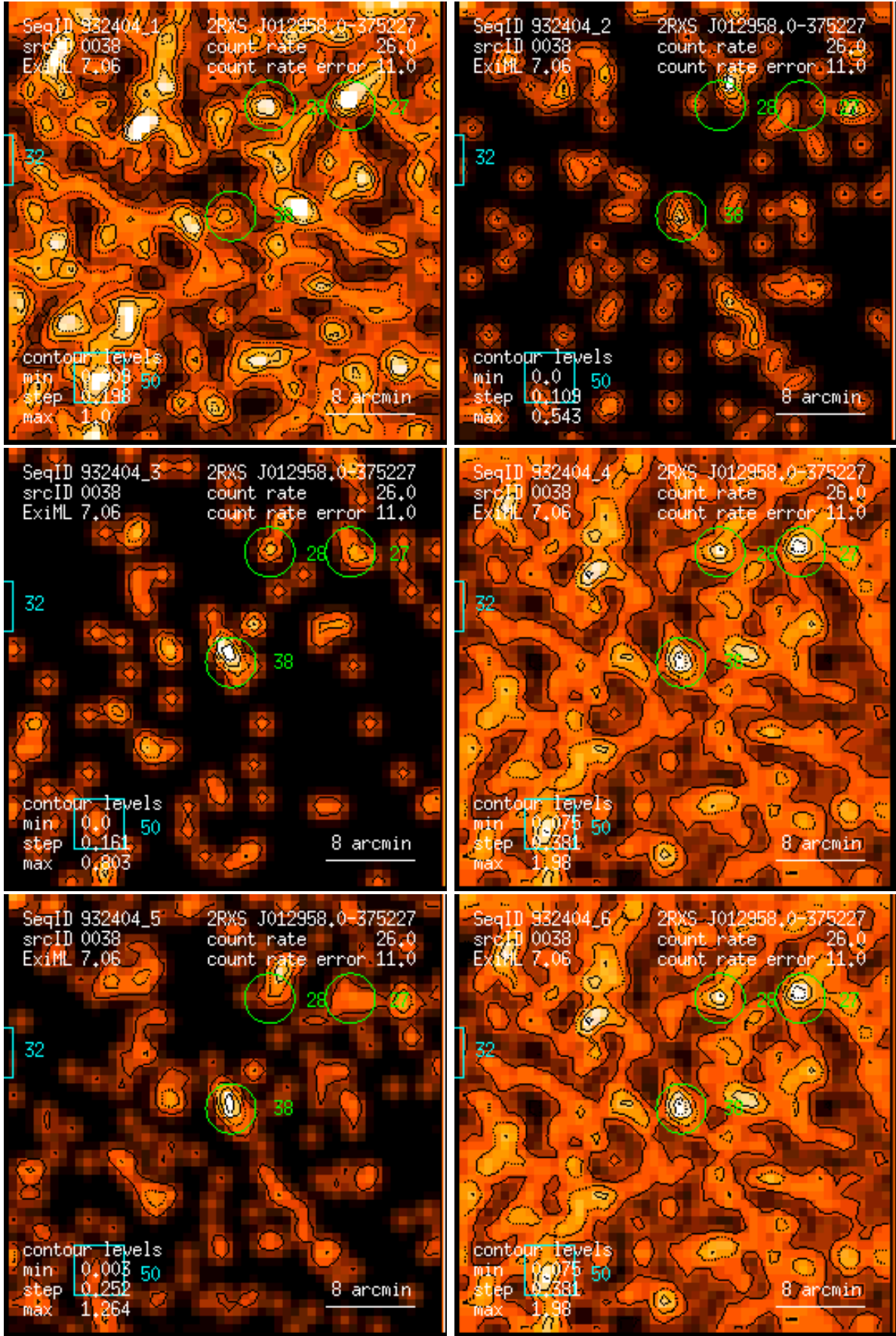
Figure 38: RASS 932404: detection 0038: band rate images, Gaussian filter: (1) PSPC channels 11 – 41, (2) 52 – 90, (3) 91 – 201, (4) 11 – 235, (5) 52 – 201, (6) 11 – 201. Broad band rates in counts/ks. Band rate contour levels in counts/ks/arcmin 2 .
