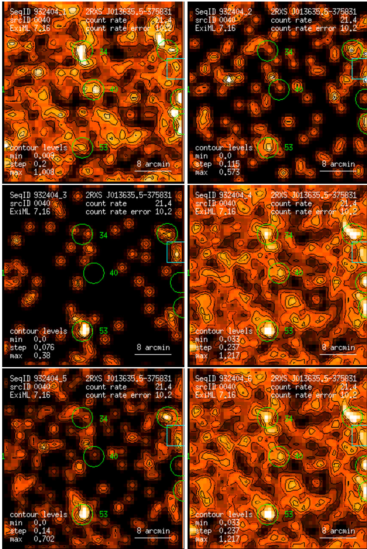
Figure 40: RASS 932404: detection 0040: band rate images, Gaussian filter: (1) PSPC channels 11 – 41, (2) 52 – 90, (3) 91 – 201, (4) 11 – 235, (5) 52 – 201, (6) 11 – 201. Broad band rates in counts/ks. Band rate contour levels in counts/ks/arcmin 2 .
