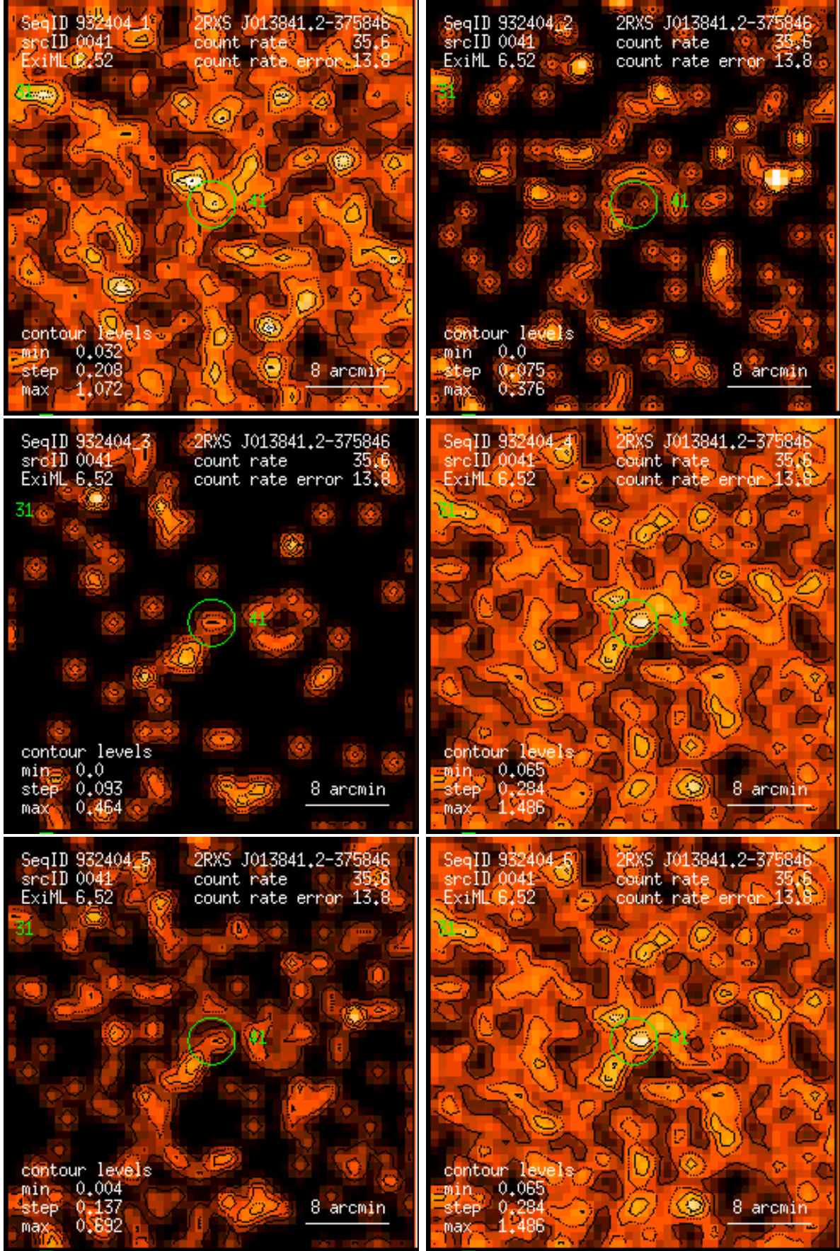
Figure 41: RASS 932404: detection 0041: band rate images, Gaussian filter: (1) PSPC channels 11 – 41, (2) 52 – 90, (3) 91 – 201, (4) 11 – 235, (5) 52 – 201, (6) 11 – 201. Broad band rates in counts/ks. Band rate contour levels in counts/ks/arcmin 2 .
