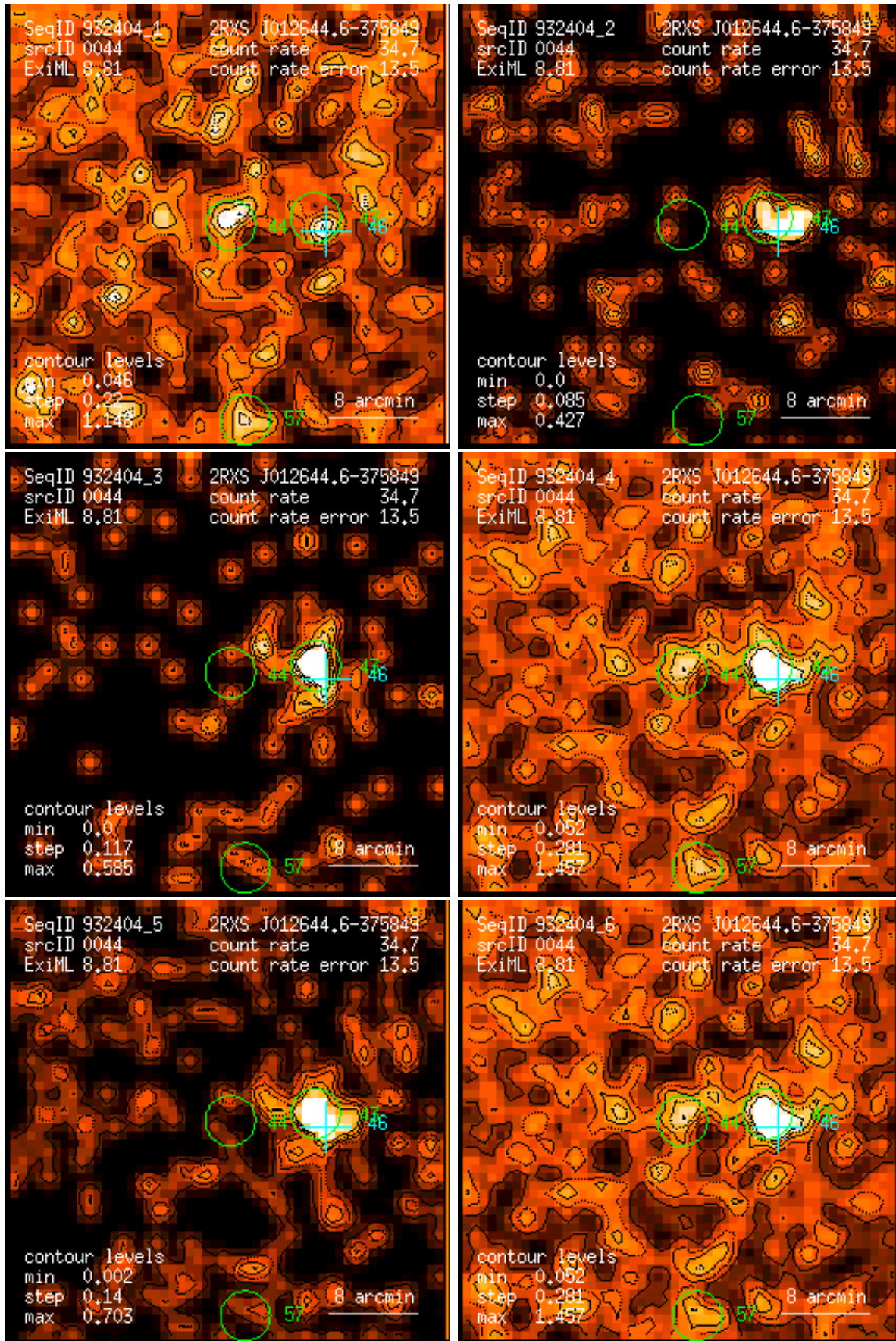
Figure 44: RASS 932404: detection 0044: band rate images, Gaussian filter: (1) PSPC channels 11 – 41, (2) 52 – 90, (3) 91 – 201, (4) 11 – 235, (5) 52 – 201, (6) 11 – 201. Broad band rates in counts/ks. Band rate contour levels in counts/ks/arcmin 2 .
