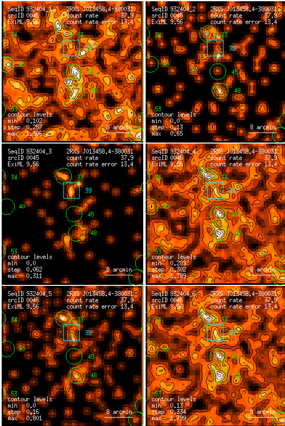
Figure 45: RASS 932404: detection 0045: band rate images, Gaussian filter: (1) PSPC channels 11 – 41, (2) 52 – 90, (3) 91 – 201, (4) 11 – 235, (5) 52 – 201, (6) 11 – 201. Broad band rates in counts/ks. Band rate contour levels in counts/ks/arcmin 2 .
