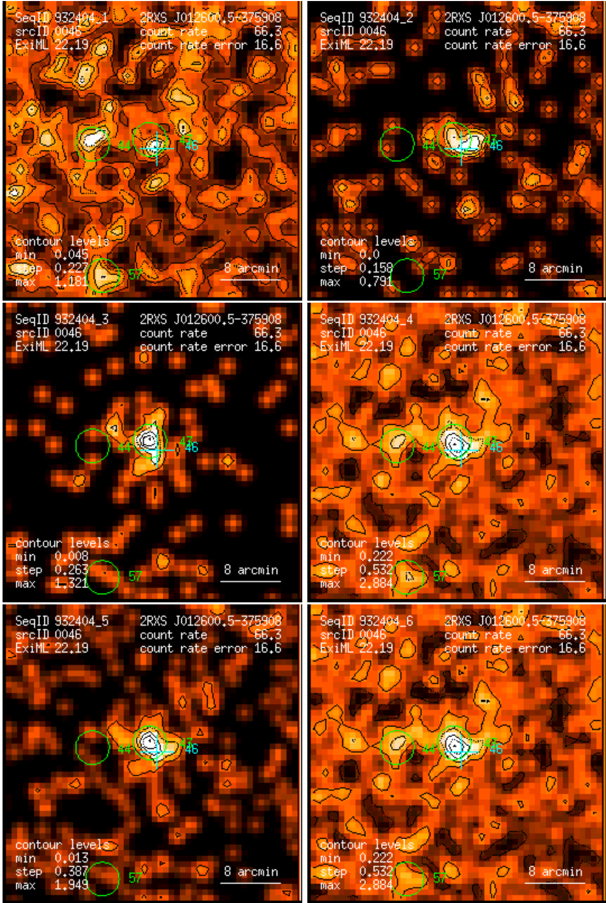
Figure 46: RASS 932404: detection 0046: band rate images, Gaussian filter: (1) PSPC channels 11 – 41, (2) 52 – 90, (3) 91 – 201, (4) 11 – 235, (5) 52 – 201, (6) 11 – 201. Broad band rates in counts/ks. Band rate contour levels in counts/ks/arcmin 2 .
