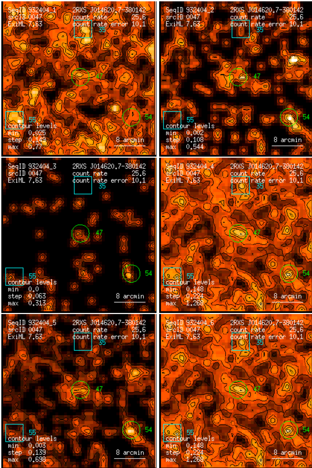
Figure 47: RASS 932404: detection 0047: band rate images, Gaussian filter: (1) PSPC channels 11 – 41, (2) 52 – 90, (3) 91 – 201, (4) 11 – 235, (5) 52 – 201, (6) 11 – 201. Broad band rates in counts/ks. Band rate contour levels in counts/ks/arcmin 2 .
