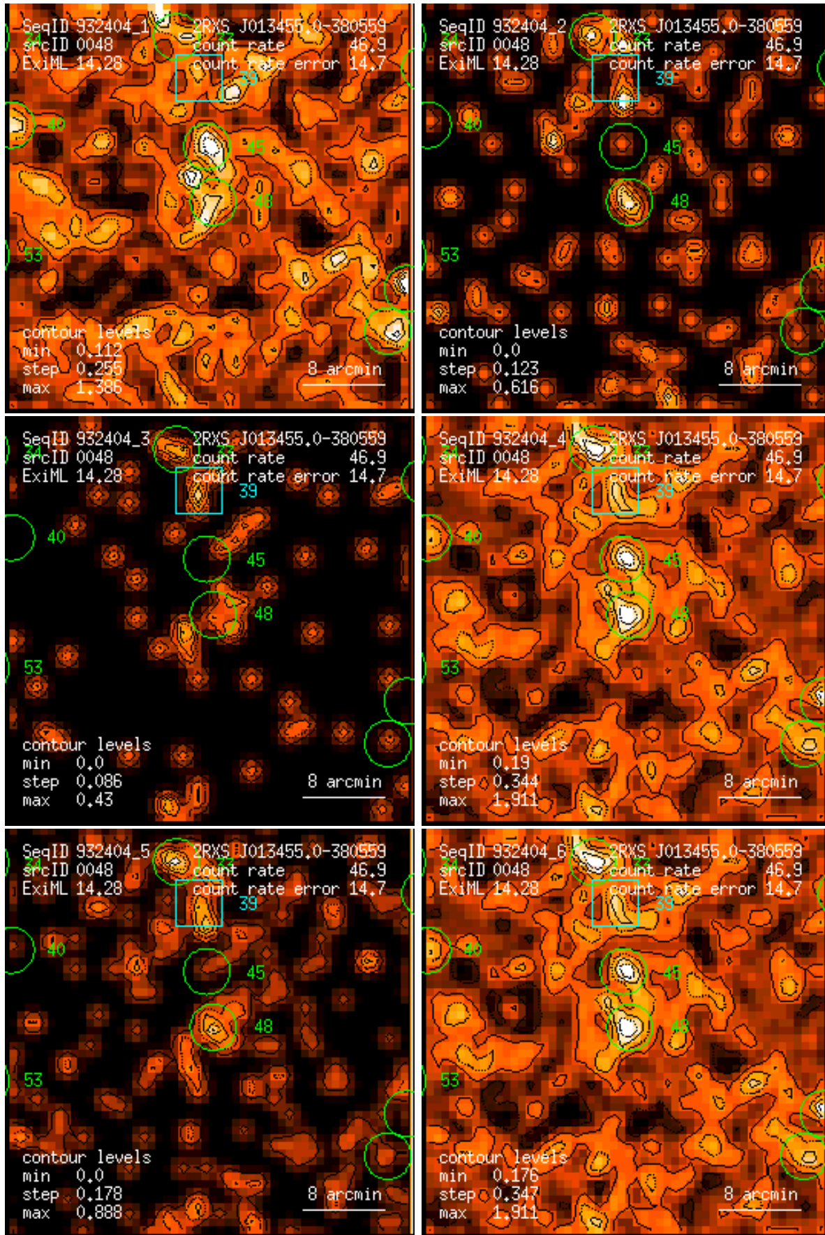
Figure 48: RASS 932404: detection 0048: band rate images, Gaussian filter: (1) PSPC channels 11 – 41, (2) 52 – 90, (3) 91 – 201, (4) 11 – 235, (5) 52 – 201, (6) 11 – 201. Broad band rates in counts/ks. Band rate contour levels in counts/ks/arcmin 2 .
