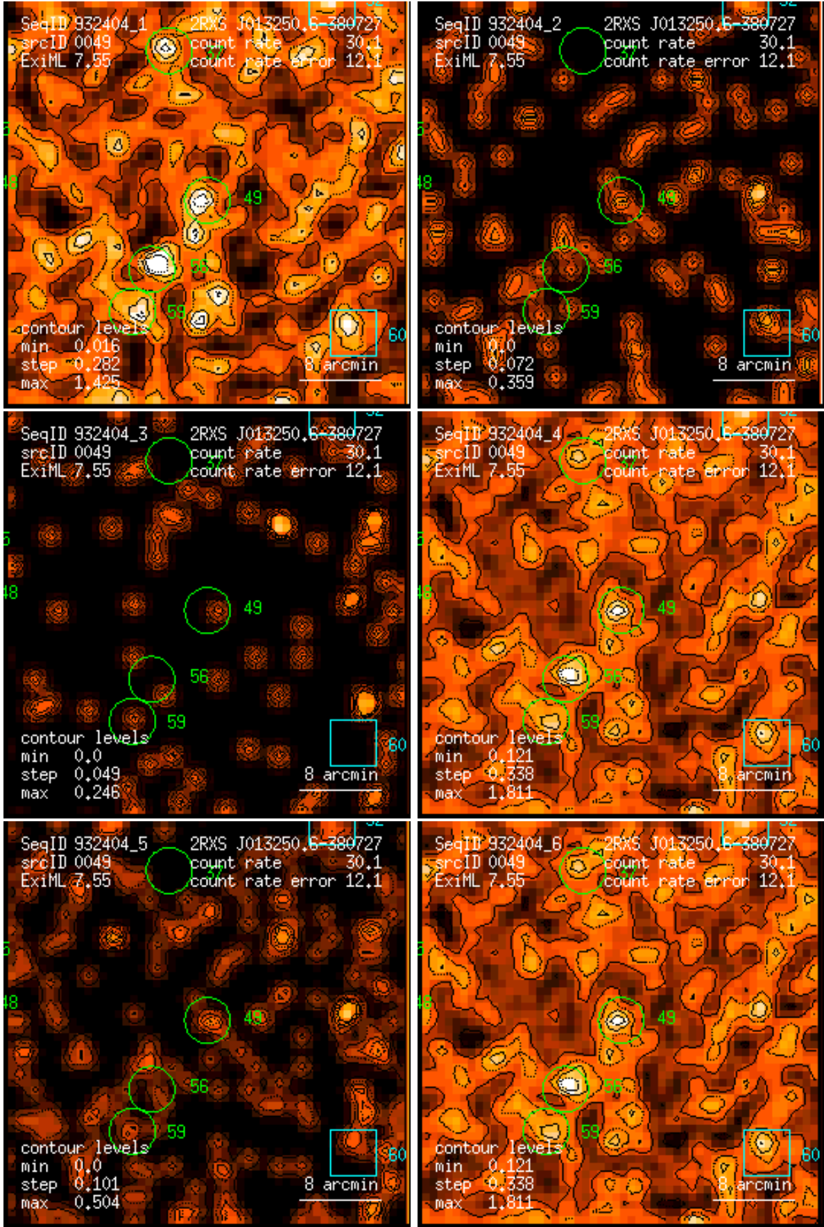
Figure 49: RASS 932404: detection 0049: band rate images, Gaussian filter: (1) PSPC channels 11 – 41, (2) 52 – 90, (3) 91 – 201, (4) 11 – 235, (5) 52 – 201, (6) 11 – 201. Broad band rates in counts/ks. Band rate contour levels in counts/ks/arcmin 2 .
