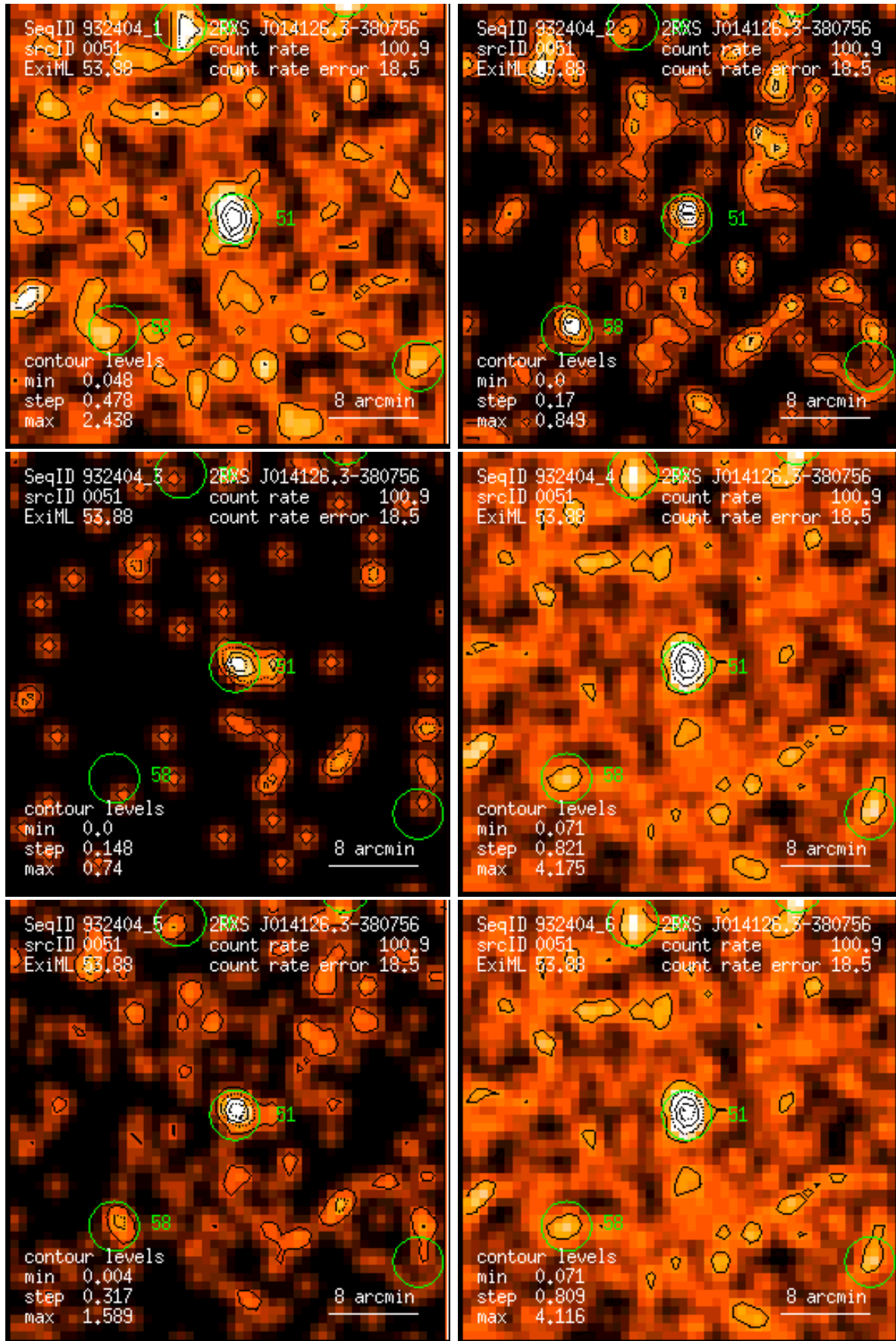
Figure 51: RASS 932404: detection 0051: band rate images, Gaussian filter: (1) PSPC channels 11 – 41, (2) 52 – 90, (3) 91 – 201, (4) 11 – 235, (5) 52 – 201, (6) 11 – 201. Broad band rates in counts/ks. Band rate contour levels in counts/ks/arcmin 2 .
