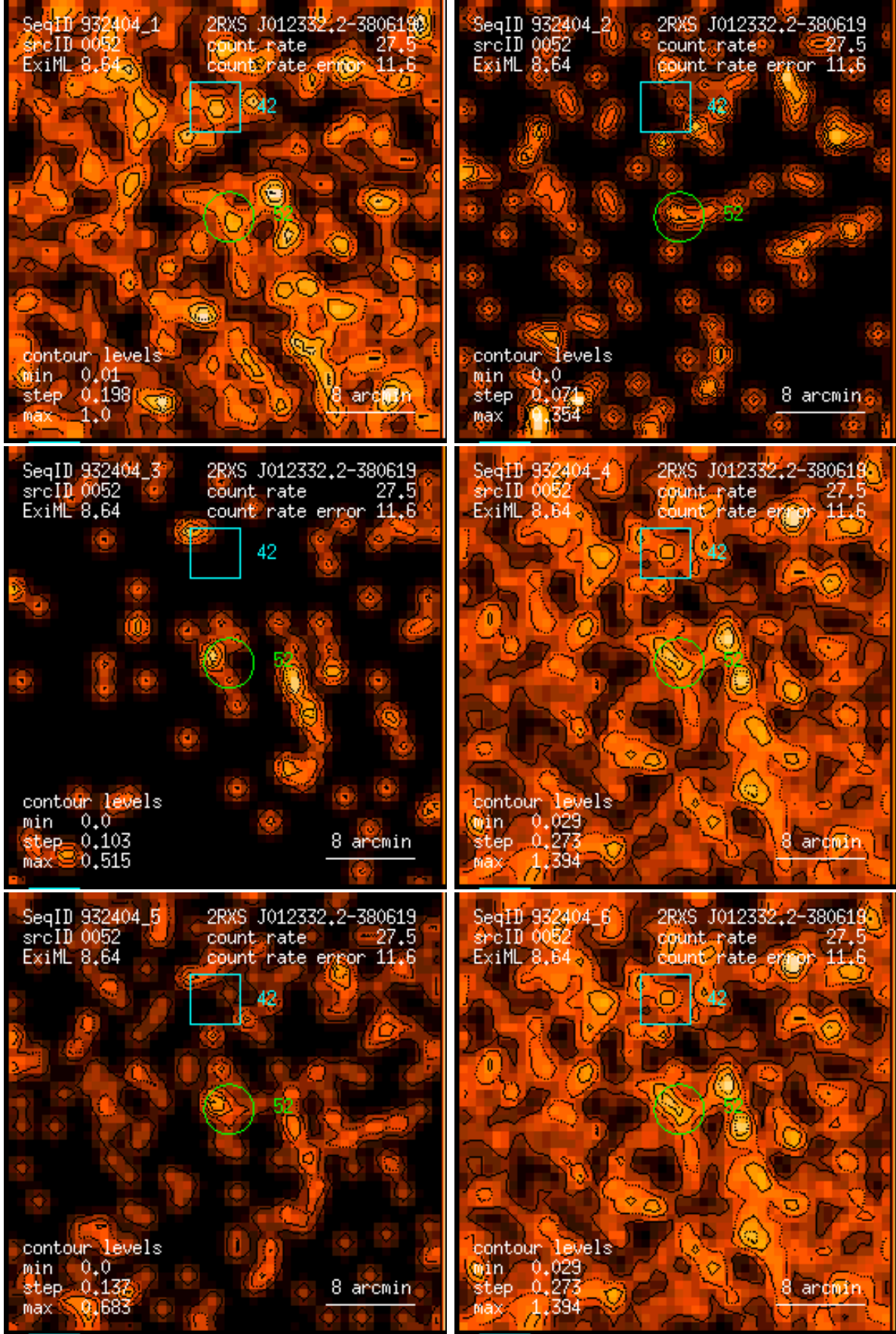
Figure 52: RASS 932404: detection 0052: band rate images, Gaussian filter: (1) PSPC channels 11 – 41, (2) 52 – 90, (3) 91 – 201, (4) 11 – 235, (5) 52 – 201, (6) 11 – 201. Broad band rates in counts/ks. Band rate contour levels in counts/ks/arcmin 2 .
