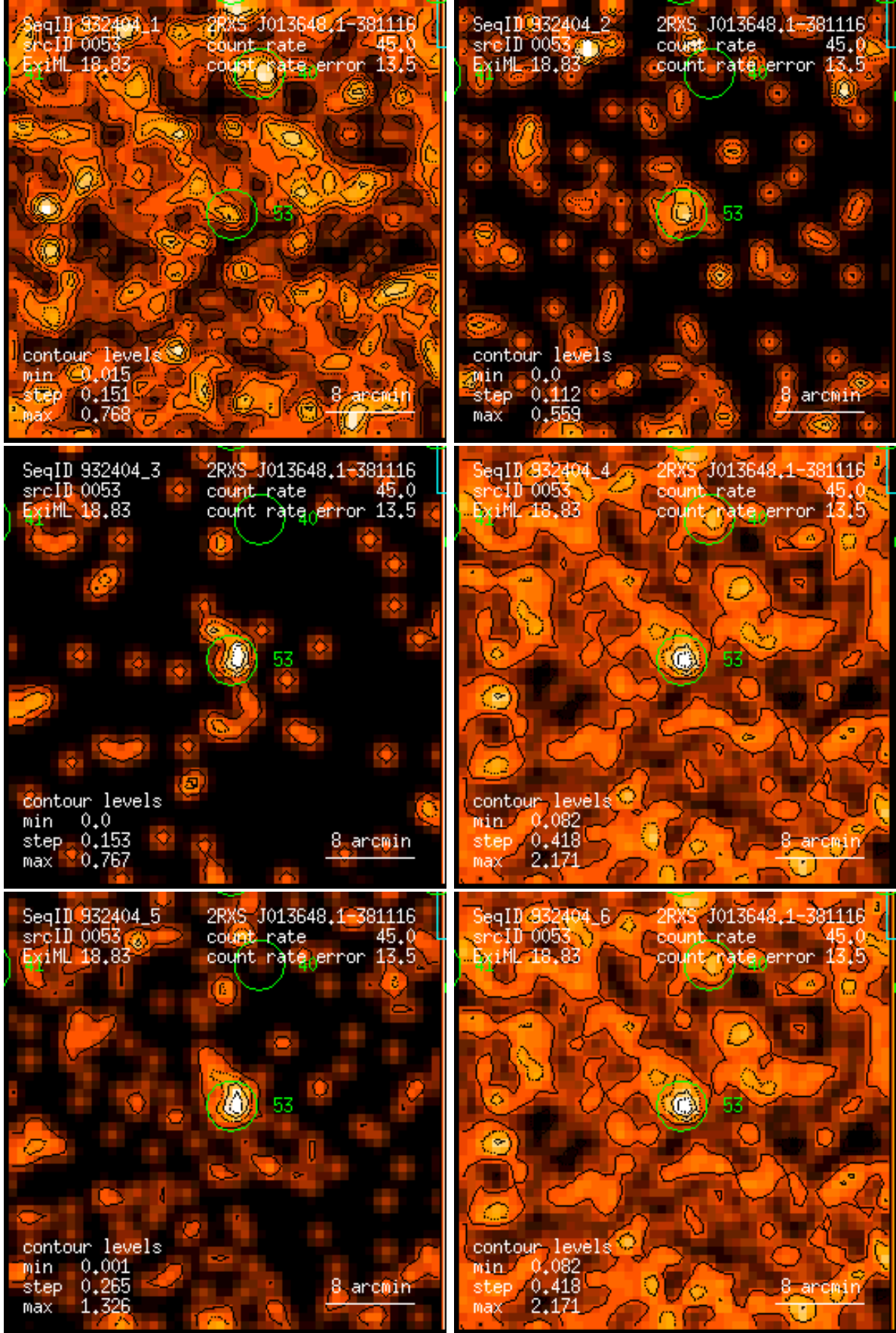
Figure 53: RASS 932404: detection 0053: band rate images, Gaussian filter: (1) PSPC channels 11 – 41, (2) 52 – 90, (3) 91 – 201, (4) 11 – 235, (5) 52 – 201, (6) 11 – 201. Broad band rates in counts/ks. Band rate contour levels in counts/ks/arcmin 2 .
