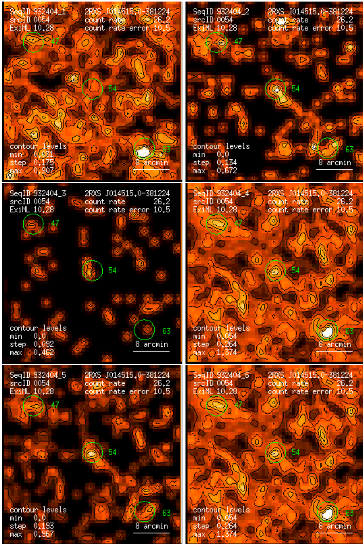
Figure 54: RASS 932404: detection 0054: band rate images, Gaussian filter: (1) PSPC channels 11 – 41, (2) 52 – 90, (3) 91 – 201, (4) 11 – 235, (5) 52 – 201, (6) 11 – 201. Broad band rates in counts/ks. Band rate contour levels in counts/ks/arcmin 2 .
