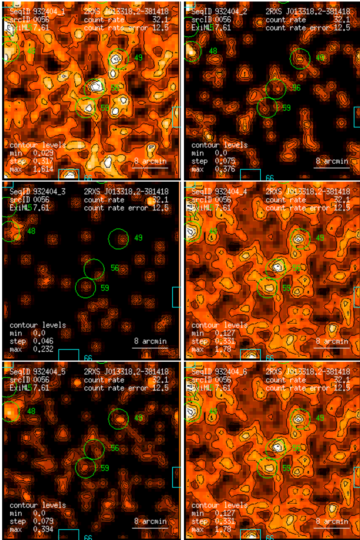
Figure 56: RASS 932404: detection 0056: band rate images, Gaussian filter: (1) PSPC channels 11 – 41, (2) 52 – 90, (3) 91 – 201, (4) 11 – 235, (5) 52 – 201, (6) 11 – 201. Broad band rates in counts/ks. Band rate contour levels in counts/ks/arcmin 2 .
