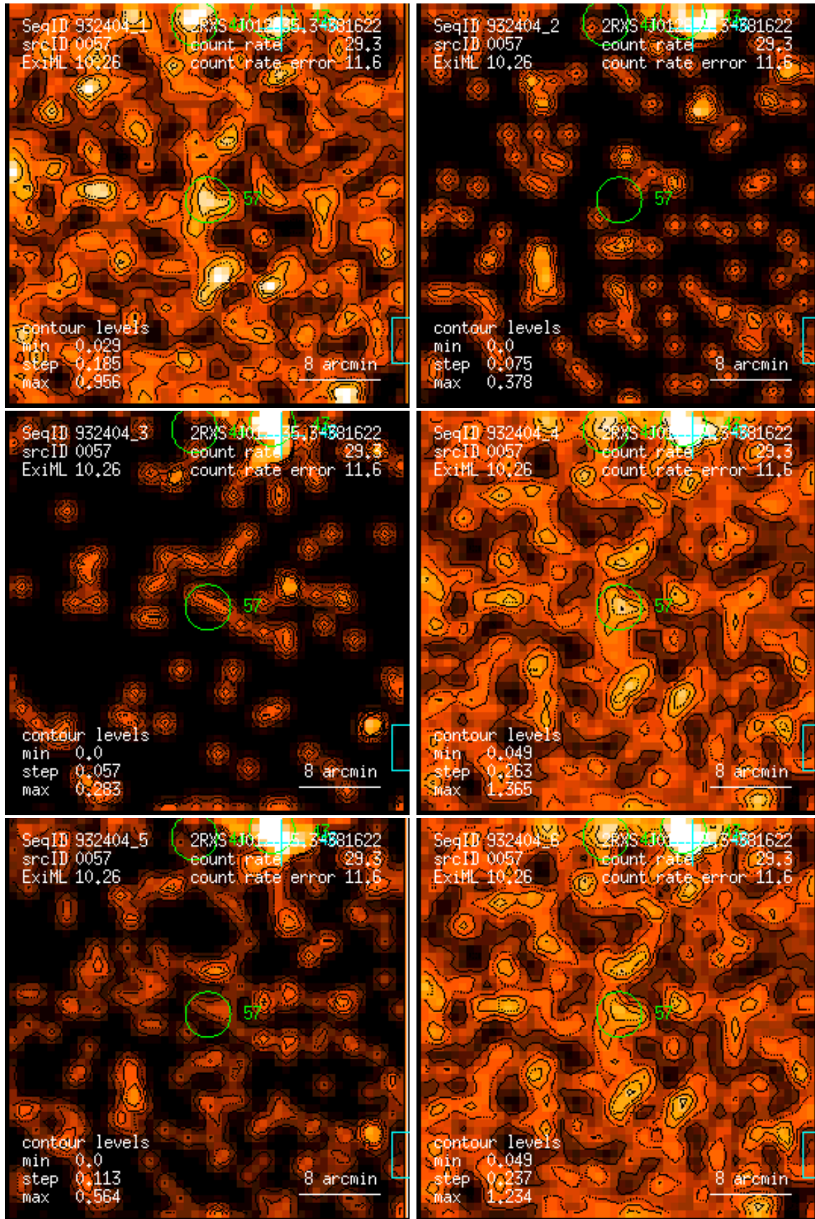
Figure 57: RASS 932404: detection 0057: band rate images, Gaussian filter: (1) PSPC channels 11 – 41, (2) 52 – 90, (3) 91 – 201, (4) 11 – 235, (5) 52 – 201, (6) 11 – 201. Broad band rates in counts/ks. Band rate contour levels in counts/ks/arcmin 2 .
