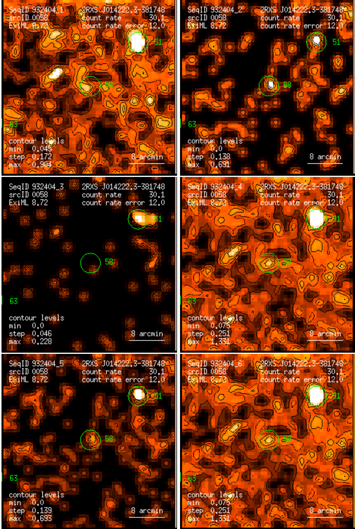
Figure 58: RASS 932404: detection 0058: band rate images, Gaussian filter: (1) PSPC channels 11 – 41, (2) 52 – 90, (3) 91 – 201, (4) 11 – 235, (5) 52 – 201, (6) 11 – 201. Broad band rates in counts/ks. Band rate contour levels in counts/ks/arcmin 2 .
