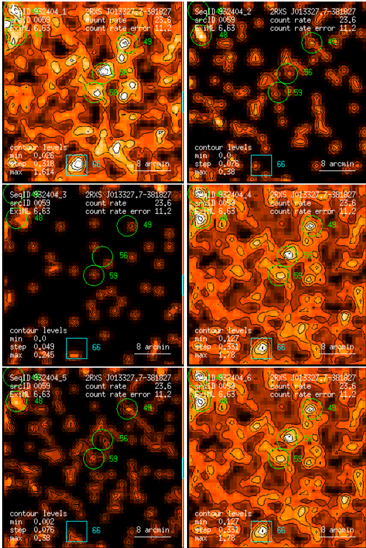
Figure 59: RASS 932404: detection 0059: band rate images, Gaussian filter: (1) PSPC channels 11 – 41, (2) 52 – 90, (3) 91 – 201, (4) 11 – 235, (5) 52 – 201, (6) 11 – 201. Broad band rates in counts/ks. Band rate contour levels in counts/ks/arcmin 2 .
