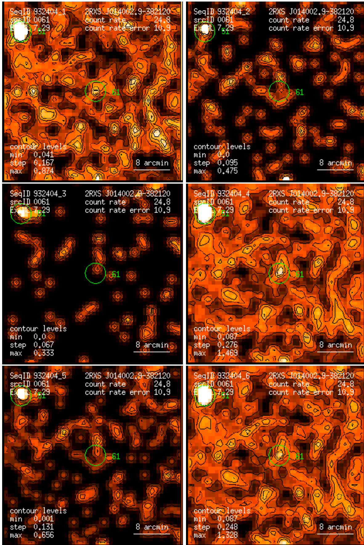
Figure 61: RASS 932404: detection 0061: band rate images, Gaussian filter: (1) PSPC channels 11 – 41, (2) 52 – 90, (3) 91 – 201, (4) 11 – 235, (5) 52 – 201, (6) 11 – 201. Broad band rates in counts/ks. Band rate contour levels in counts/ks/arcmin 2 .
