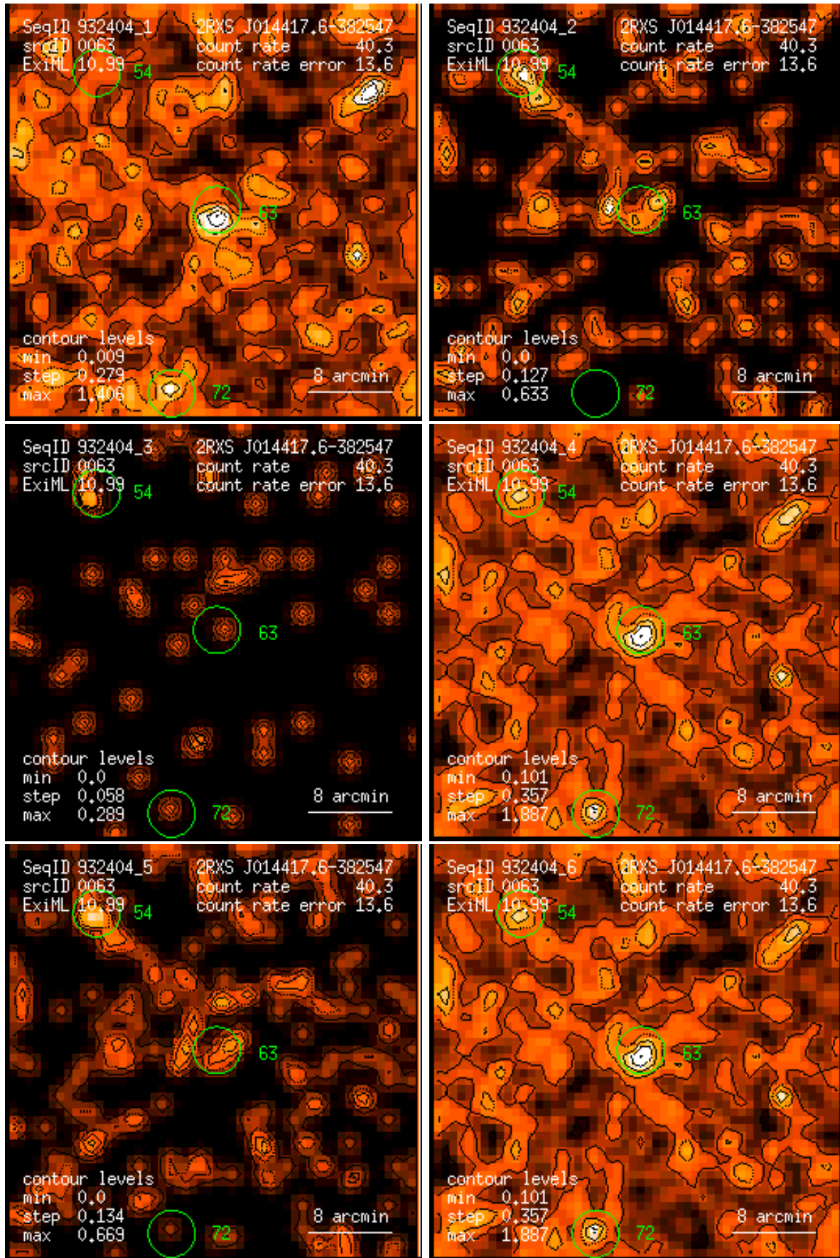
Figure 63: RASS 932404: detection 0063: band rate images, Gaussian filter: (1) PSPC channels 11 – 41, (2) 52 – 90, (3) 91 – 201, (4) 11 – 235, (5) 52 – 201, (6) 11 – 201. Broad band rates in counts/ks. Band rate contour levels in counts/ks/arcmin 2 .
