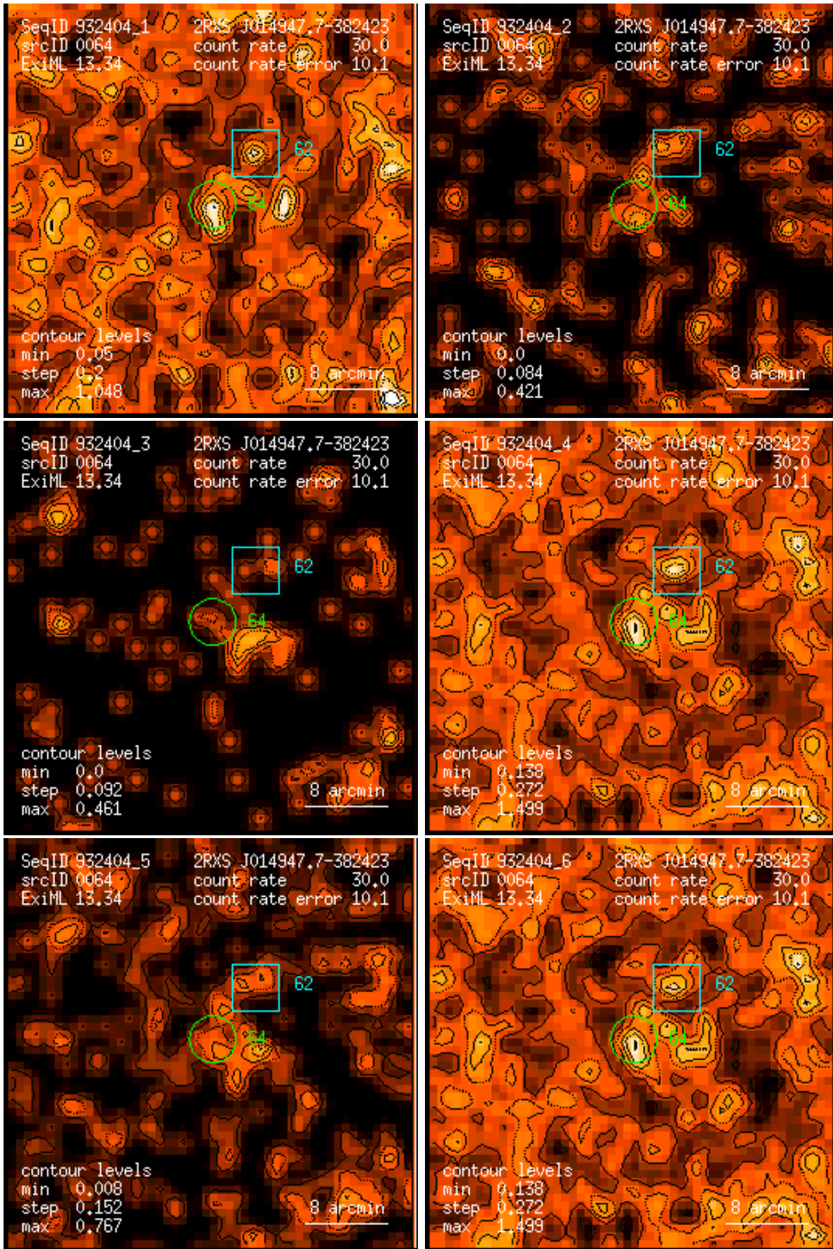
Figure 64: RASS 932404: detection 0064: band rate images, Gaussian filter: (1) PSPC channels 11 – 41, (2) 52 – 90, (3) 91 – 201, (4) 11 – 235, (5) 52 – 201, (6) 11 – 201. Broad band rates in counts/ks. Band rate contour levels in counts/ks/arcmin 2 .
