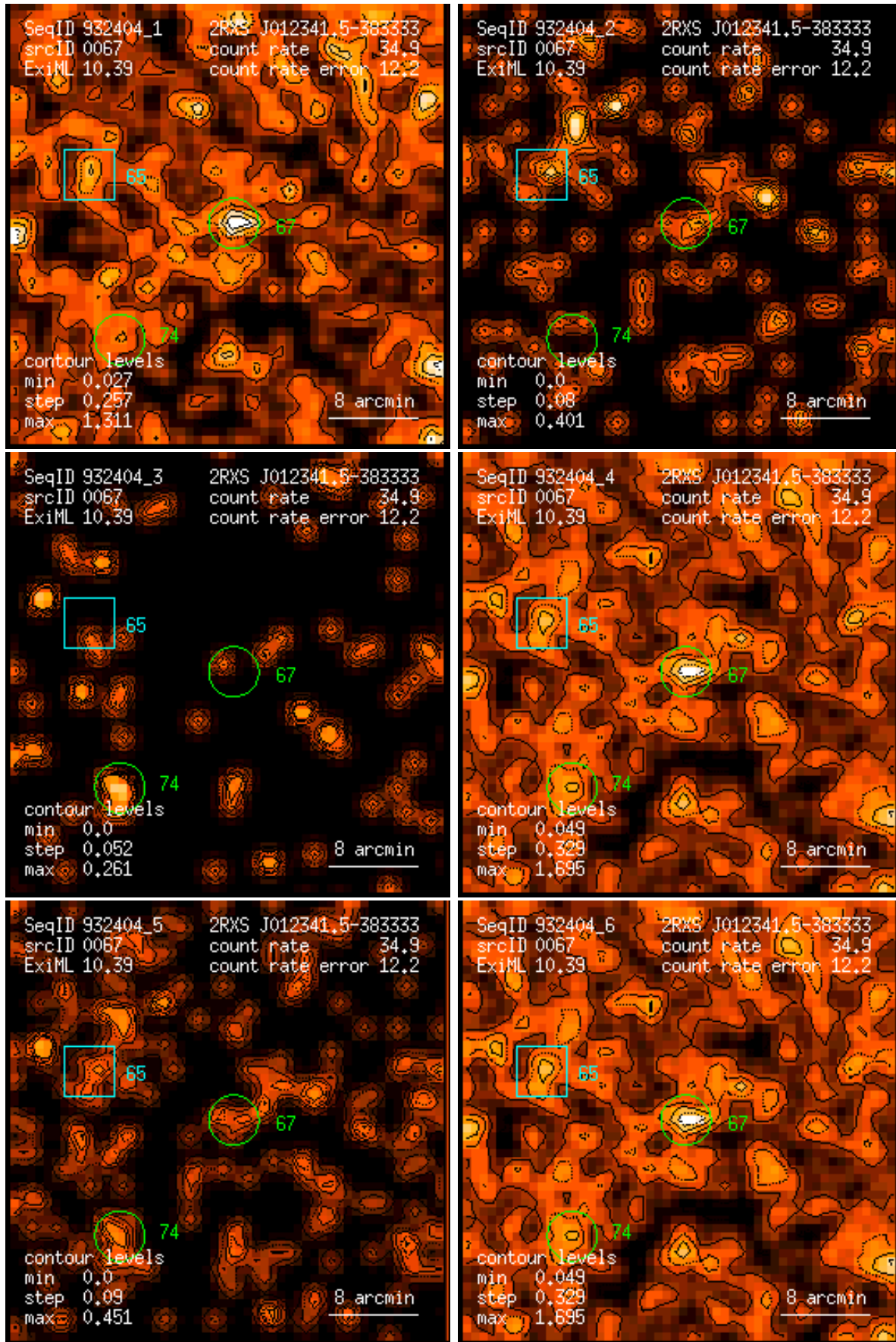
Figure 67: RASS 932404: detection 0067: band rate images, Gaussian filter: (1) PSPC channels 11 – 41, (2) 52 – 90, (3) 91 – 201, (4) 11 – 235, (5) 52 – 201, (6) 11 – 201. Broad band rates in counts/ks. Band rate contour levels in counts/ks/arcmin 2 .
