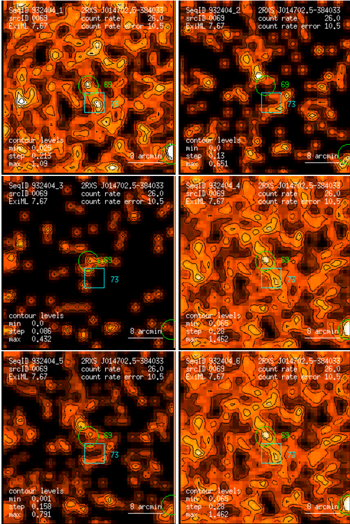
Figure 69: RASS 932404: detection 0069: band rate images, Gaussian filter: (1) PSPC channels 11 – 41, (2) 52 – 90, (3) 91 – 201, (4) 11 – 235, (5) 52 – 201, (6) 11 – 201. Broad band rates in counts/ks. Band rate contour levels in counts/ks/arcmin 2 .
