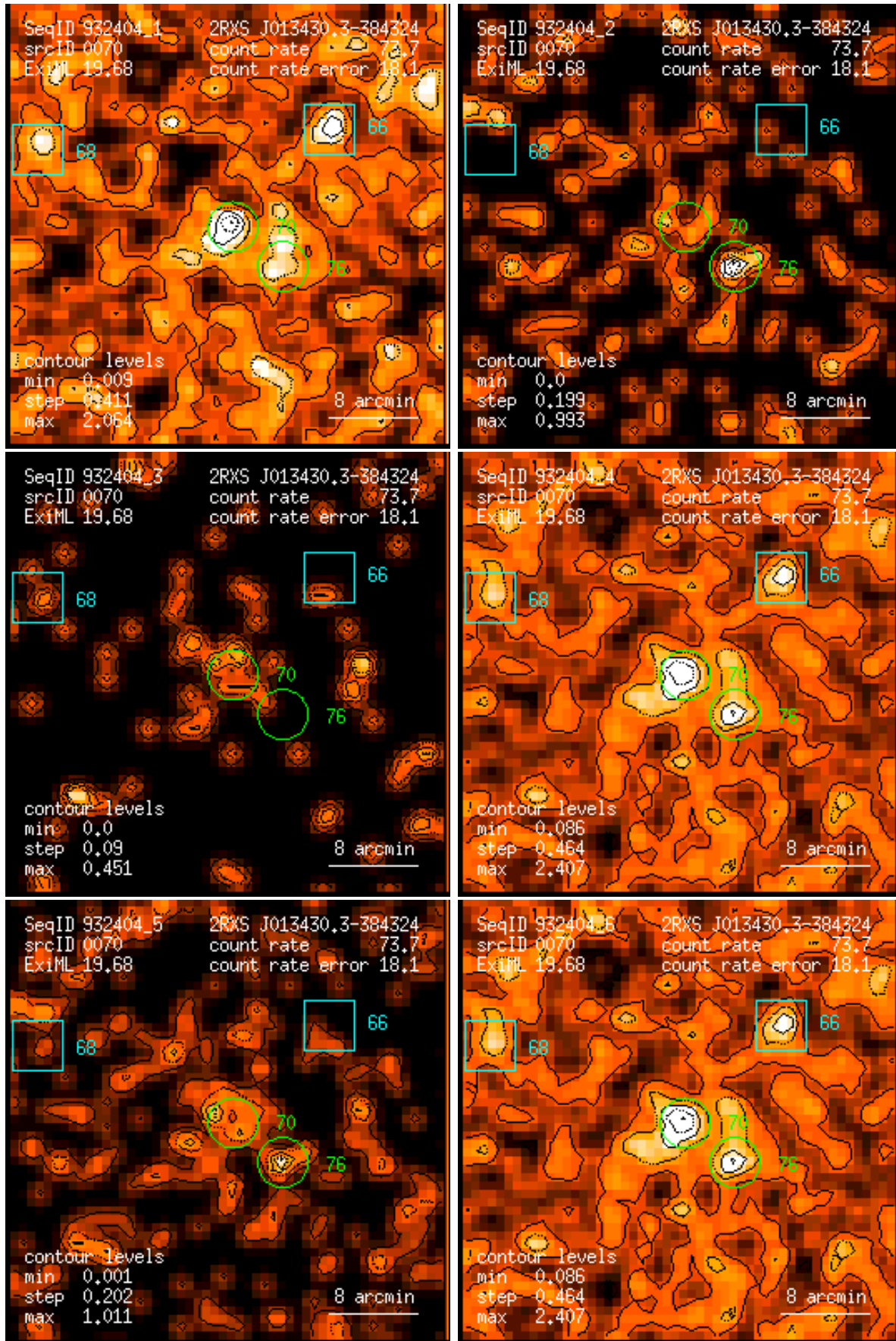
Figure 70: RASS 932404: detection 0070: band rate images, Gaussian filter: (1) PSPC channels 11 – 41, (2) 52 – 90, (3) 91 – 201, (4) 11 – 235, (5) 52 – 201, (6) 11 – 201. Broad band rates in counts/ks. Band rate contour levels in counts/ks/arcmin 2 .
