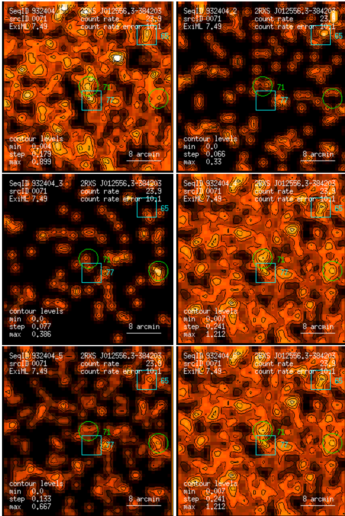
Figure 71: RASS 932404: detection 0071: band rate images, Gaussian filter: (1) PSPC channels 11 – 41, (2) 52 – 90, (3) 91 – 201, (4) 11 – 235, (5) 52 – 201, (6) 11 – 201. Broad band rates in counts/ks. Band rate contour levels in counts/ks/arcmin 2 .
