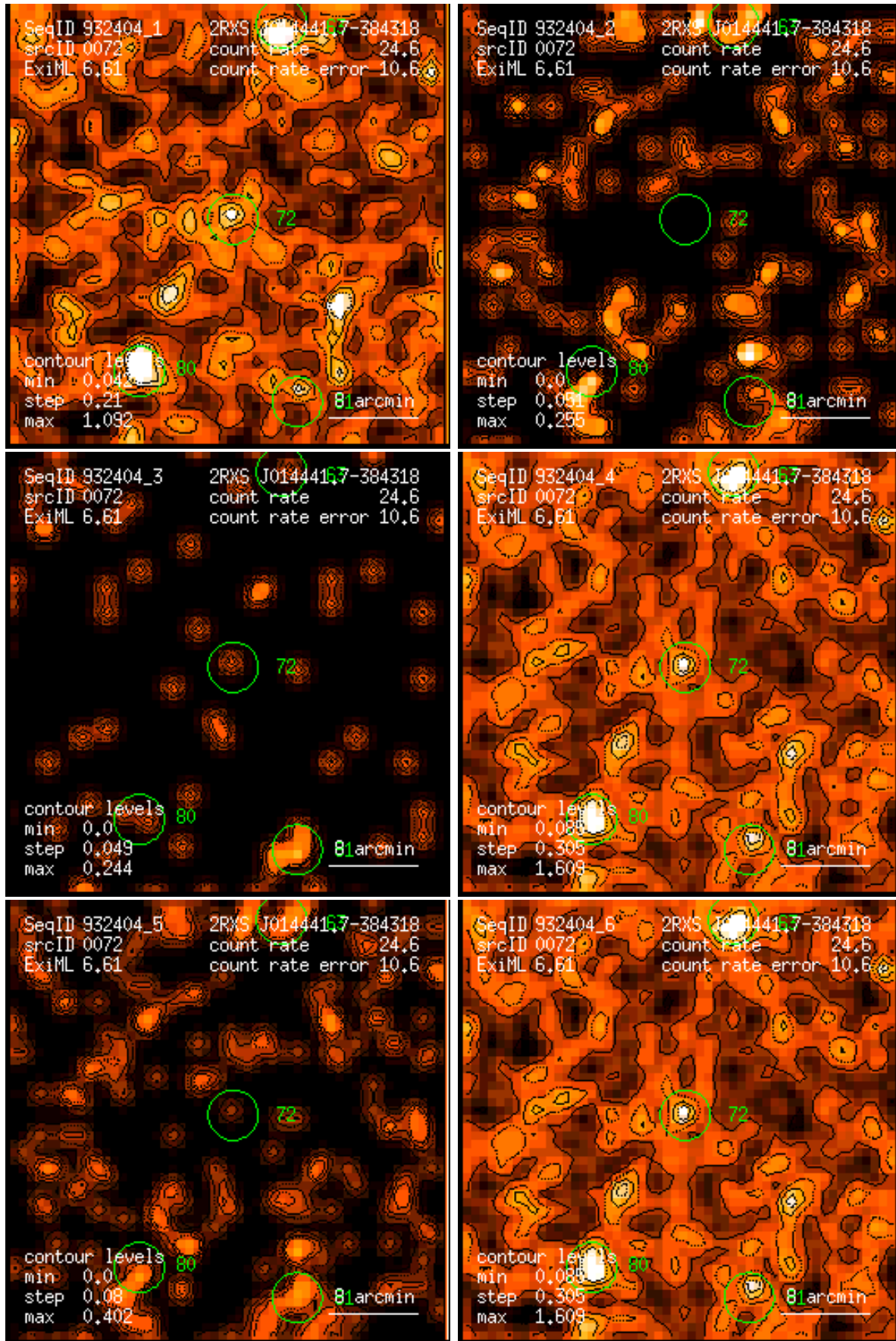
Figure 72: RASS 932404: detection 0072: band rate images, Gaussian filter: (1) PSPC channels 11 – 41, (2) 52 – 90, (3) 91 – 201, (4) 11 – 235, (5) 52 – 201, (6) 11 – 201. Broad band rates in counts/ks. Band rate contour levels in counts/ks/arcmin 2 .
