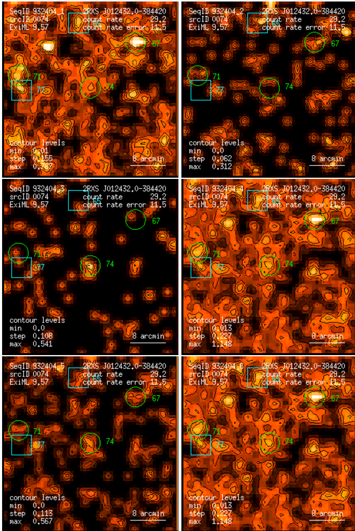
Figure 74: RASS 932404: detection 0074: band rate images, Gaussian filter: (1) PSPC channels 11 – 41, (2) 52 – 90, (3) 91 – 201, (4) 11 – 235, (5) 52 – 201, (6) 11 – 201. Broad band rates in counts/ks. Band rate contour levels in counts/ks/arcmin 2 .
