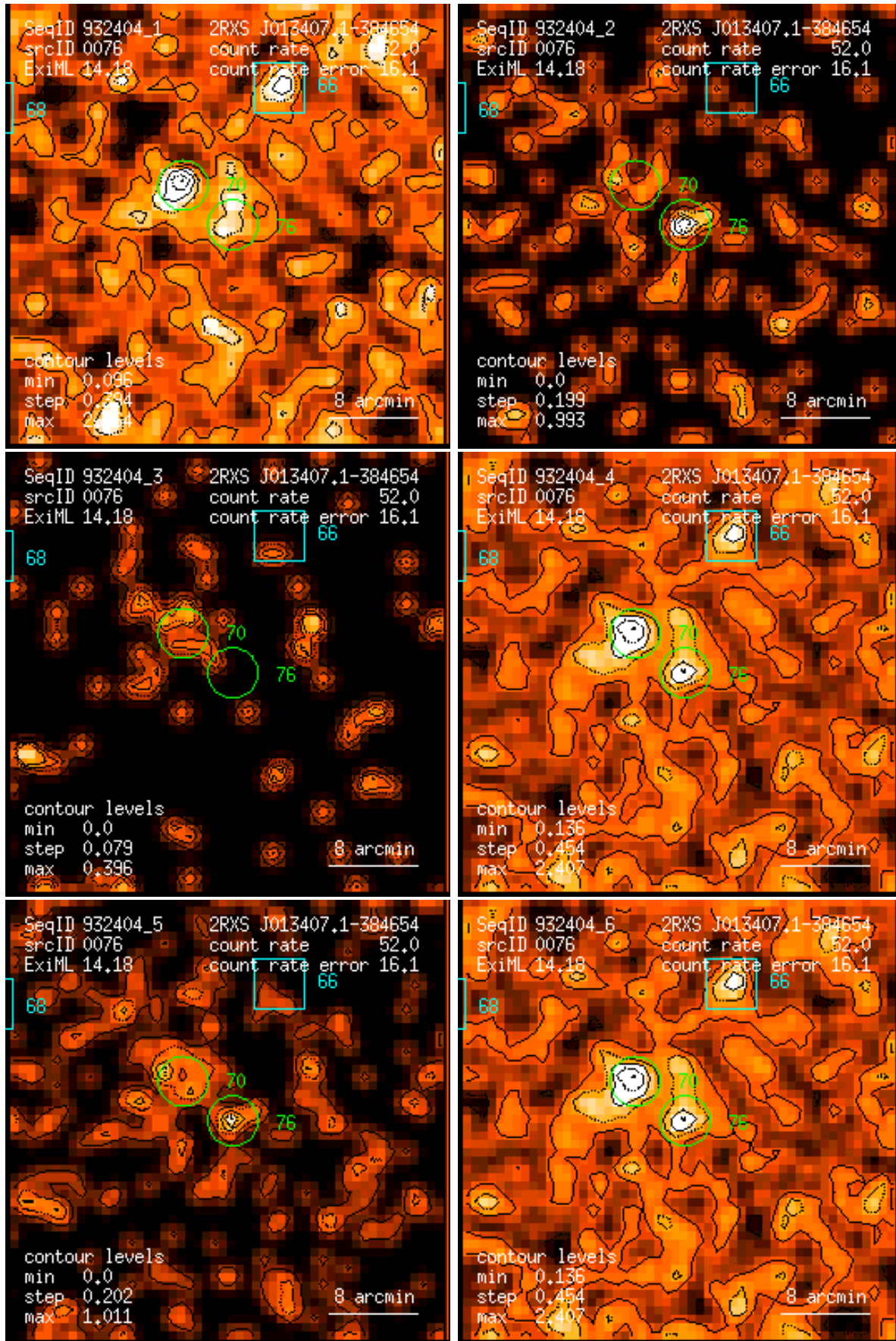
Figure 76: RASS 932404: detection 0076: band rate images, Gaussian filter: (1) PSPC channels 11 – 41, (2) 52 – 90, (3) 91 – 201, (4) 11 – 235, (5) 52 – 201, (6) 11 – 201. Broad band rates in counts/ks. Band rate contour levels in counts/ks/arcmin 2 .
