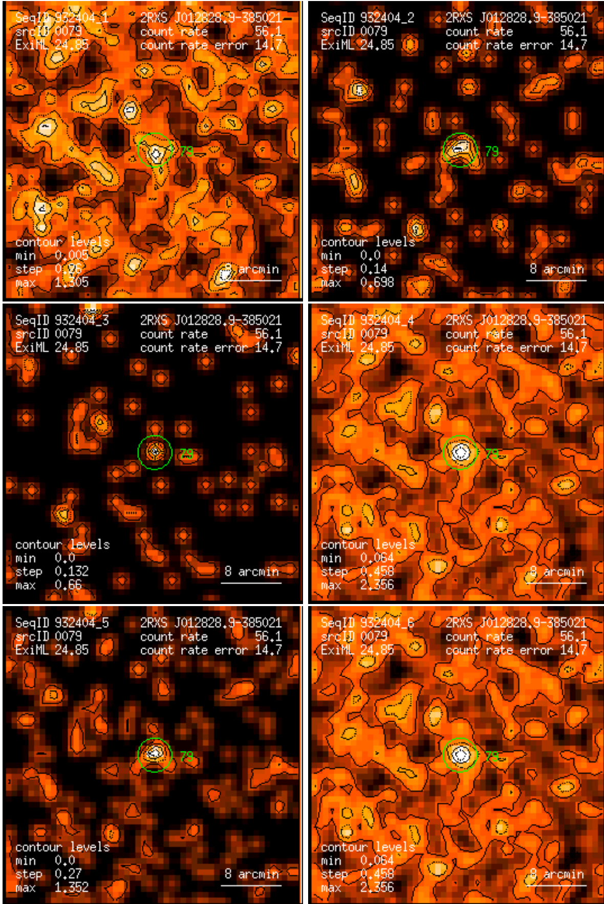
Figure 79: RASS 932404: detection 0079: band rate images, Gaussian filter: (1) PSPC channels 11 – 41, (2) 52 – 90, (3) 91 – 201, (4) 11 – 235, (5) 52 – 201, (6) 11 – 201. Broad band rates in counts/ks. Band rate contour levels in counts/ks/arcmin 2 .
