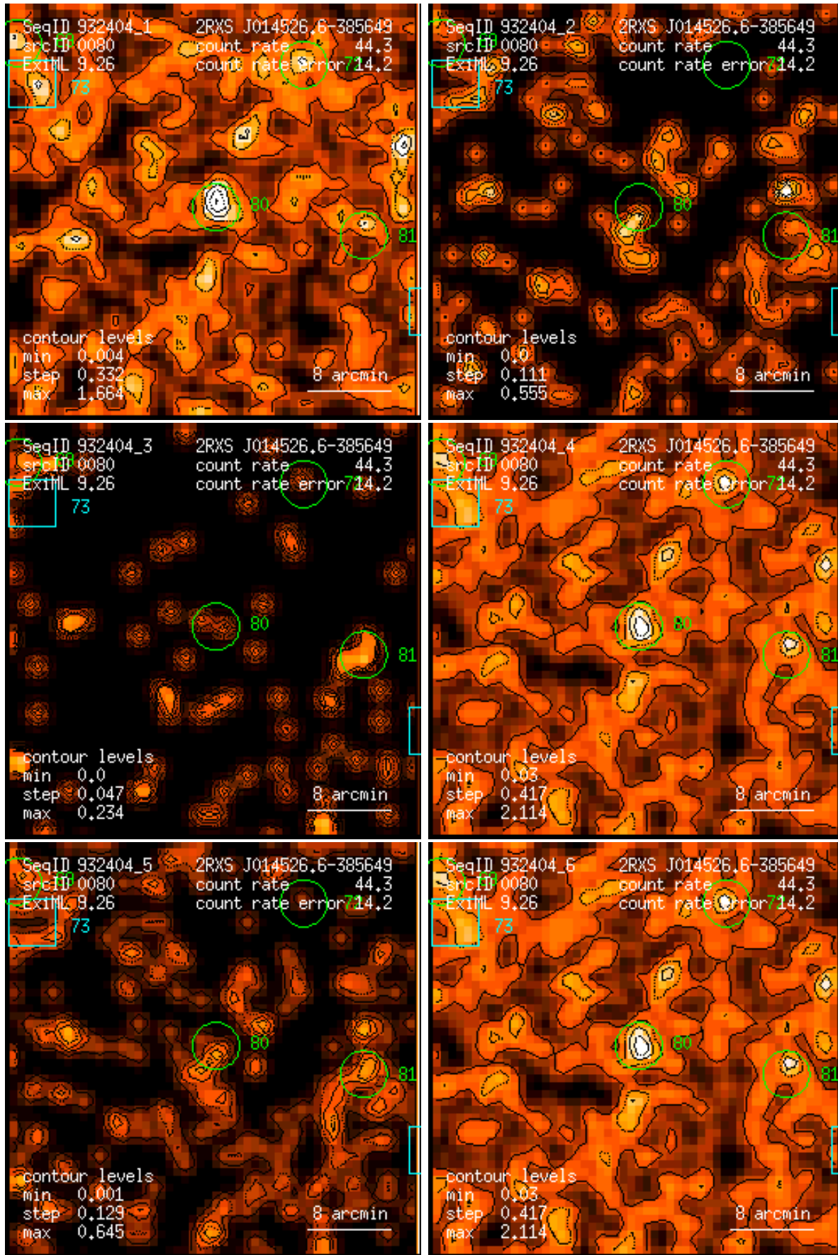
Figure 80: RASS 932404: detection 0080: band rate images, Gaussian filter: (1) PSPC channels 11 – 41, (2) 52 – 90, (3) 91 – 201, (4) 11 – 235, (5) 52 – 201, (6) 11 – 201. Broad band rates in counts/ks. Band rate contour levels in counts/ks/arcmin 2 .
