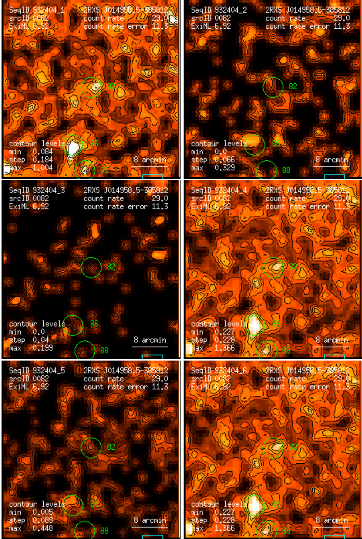
Figure 82: RASS 932404: detection 0082: band rate images, Gaussian filter: (1) PSPC channels 11 – 41, (2) 52 – 90, (3) 91 – 201, (4) 11 – 235, (5) 52 – 201, (6) 11 – 201. Broad band rates in counts/ks. Band rate contour levels in counts/ks/arcmin 2 .
