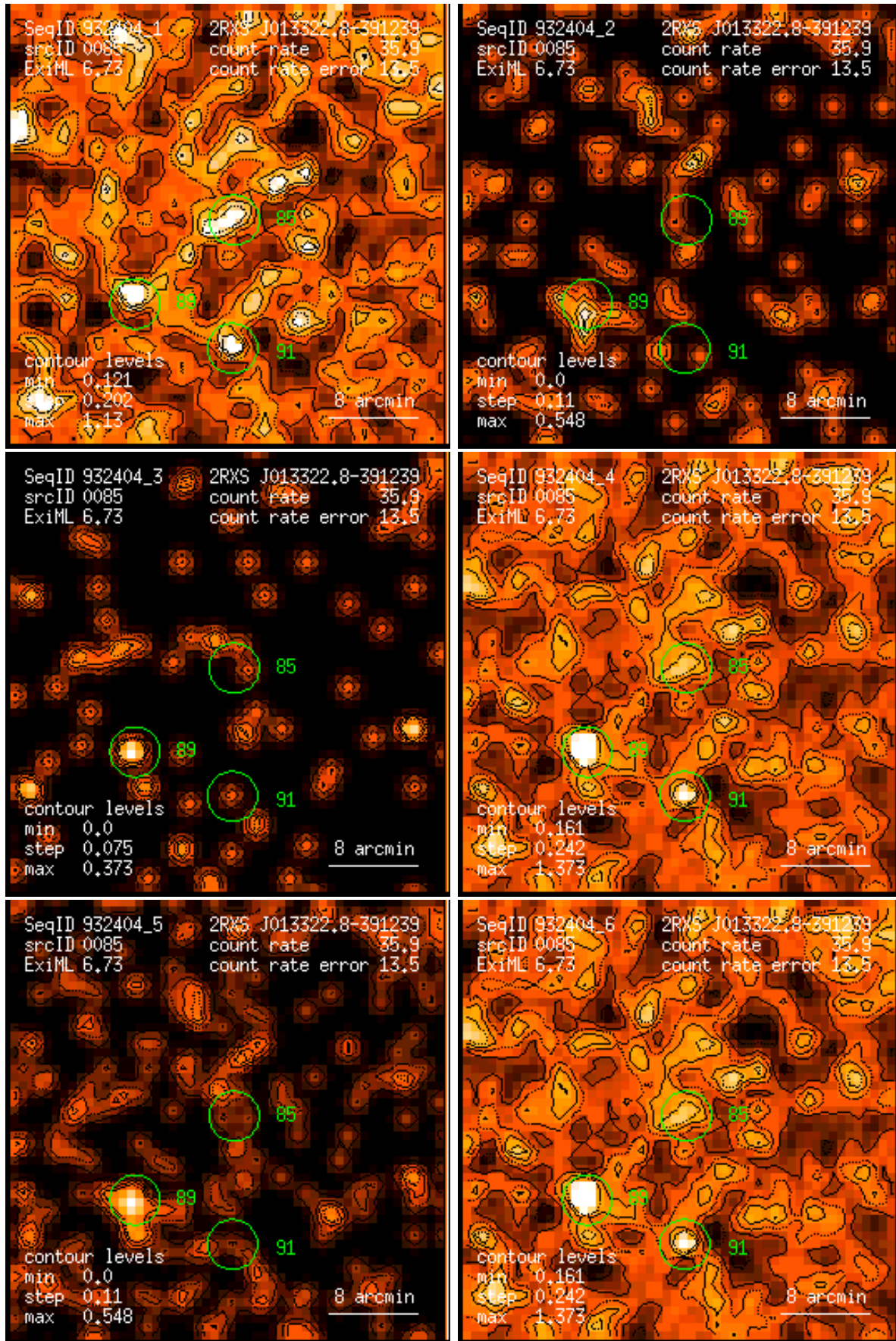
Figure 85: RASS 932404: detection 0085: band rate images, Gaussian filter: (1) PSPC channels 11 – 41, (2) 52 – 90, (3) 91 – 201, (4) 11 – 235, (5) 52 – 201, (6) 11 – 201. Broad band rates in counts/ks. Band rate contour levels in counts/ks/arcmin 2 .
