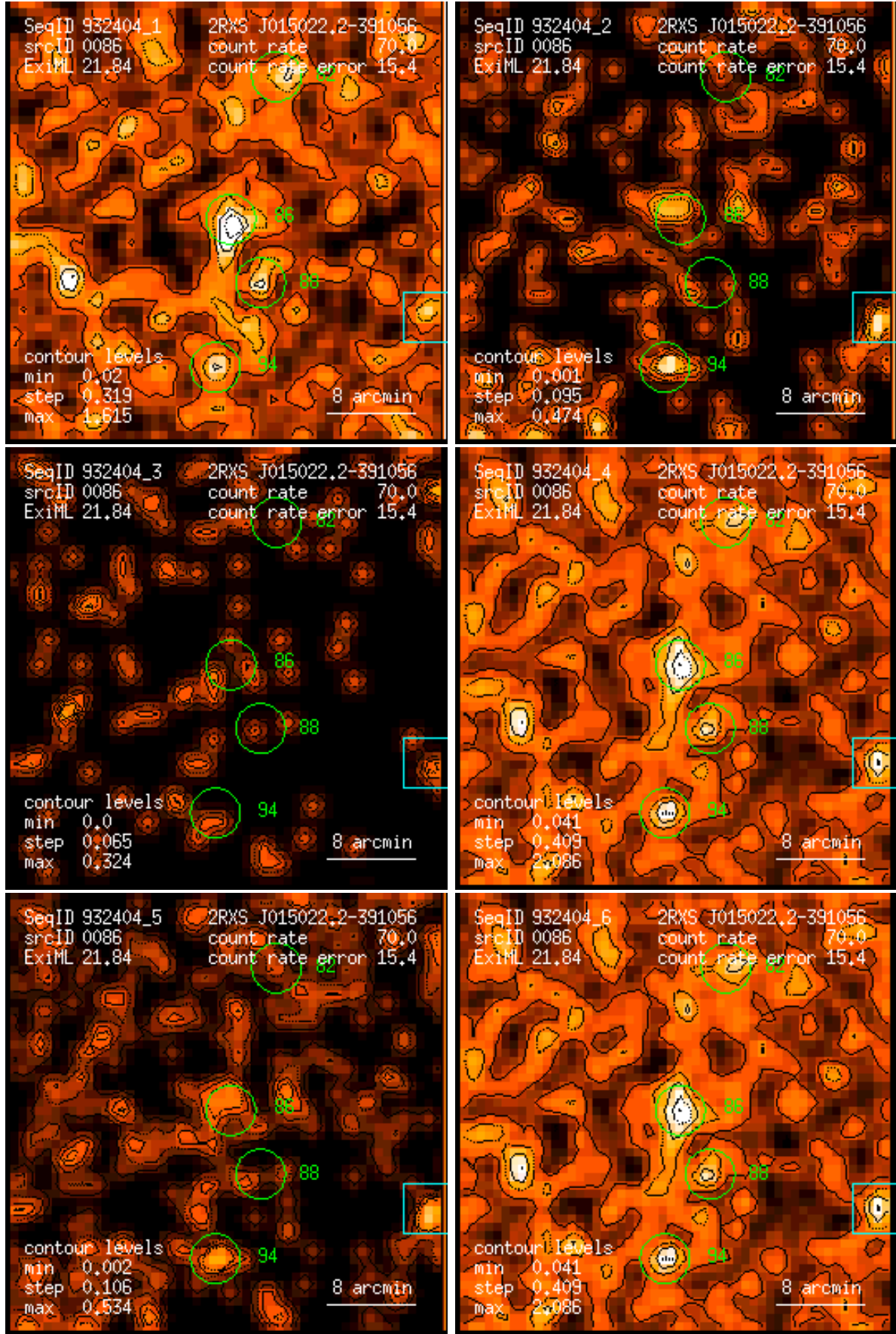
Figure 86: RASS 932404: detection 0086: band rate images, Gaussian filter: (1) PSPC channels 11 – 41, (2) 52 – 90, (3) 91 – 201, (4) 11 – 235, (5) 52 – 201, (6) 11 – 201. Broad band rates in counts/ks. Band rate contour levels in counts/ks/arcmin 2 .
