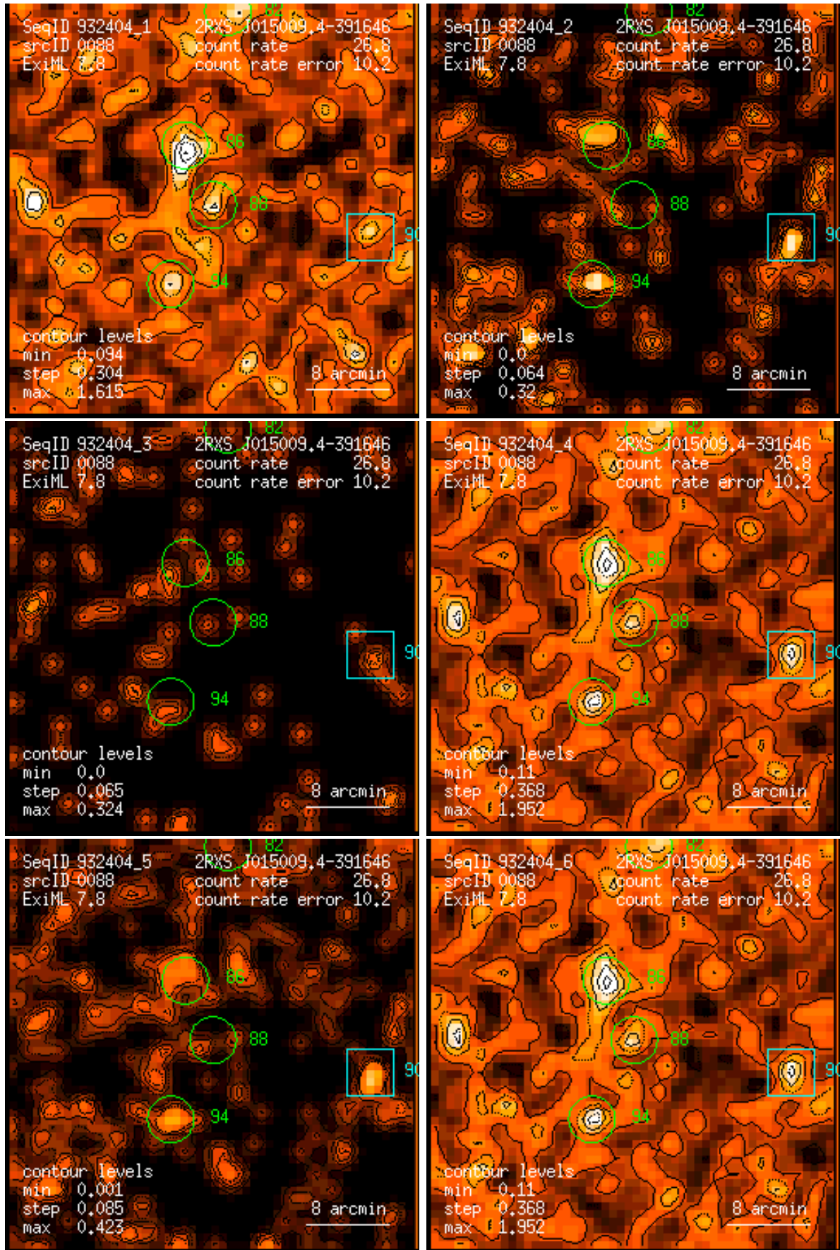
Figure 88: RASS 932404: detection 0088: band rate images, Gaussian filter: (1) PSPC channels 11 – 41, (2) 52 – 90, (3) 91 – 201, (4) 11 – 235, (5) 52 – 201, (6) 11 – 201. Broad band rates in counts/ks. Band rate contour levels in counts/ks/arcmin 2 .
